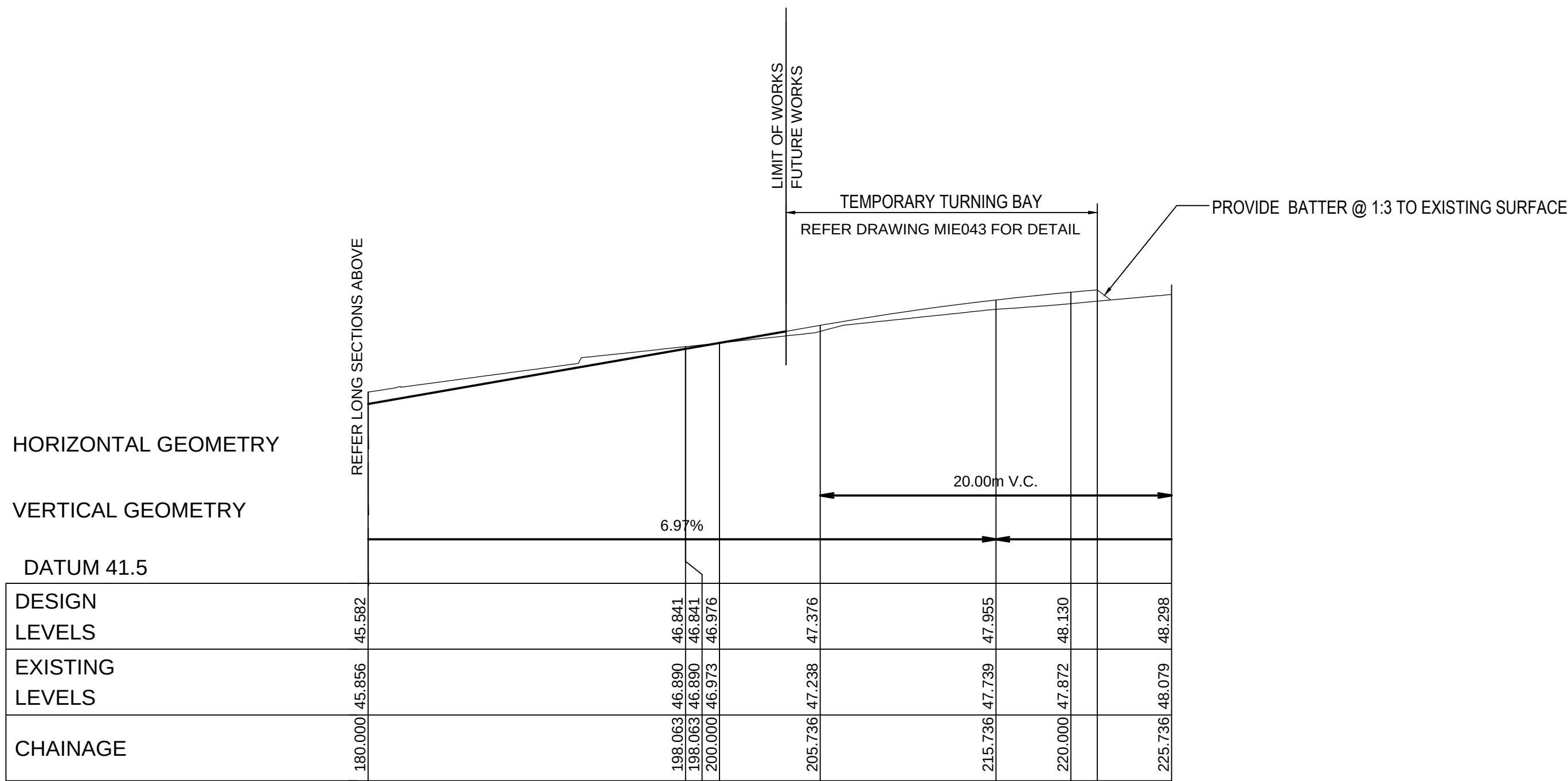
LONGITUDINAL ROAD No. 12 HORIZONTAL SCALE 1:250
