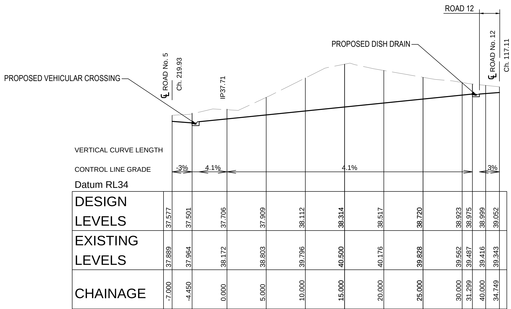
LONGITUDINAL ROAD No. 13 HORIZONTAL SCALE 1:250 VERTICAL SCALE 1:100
