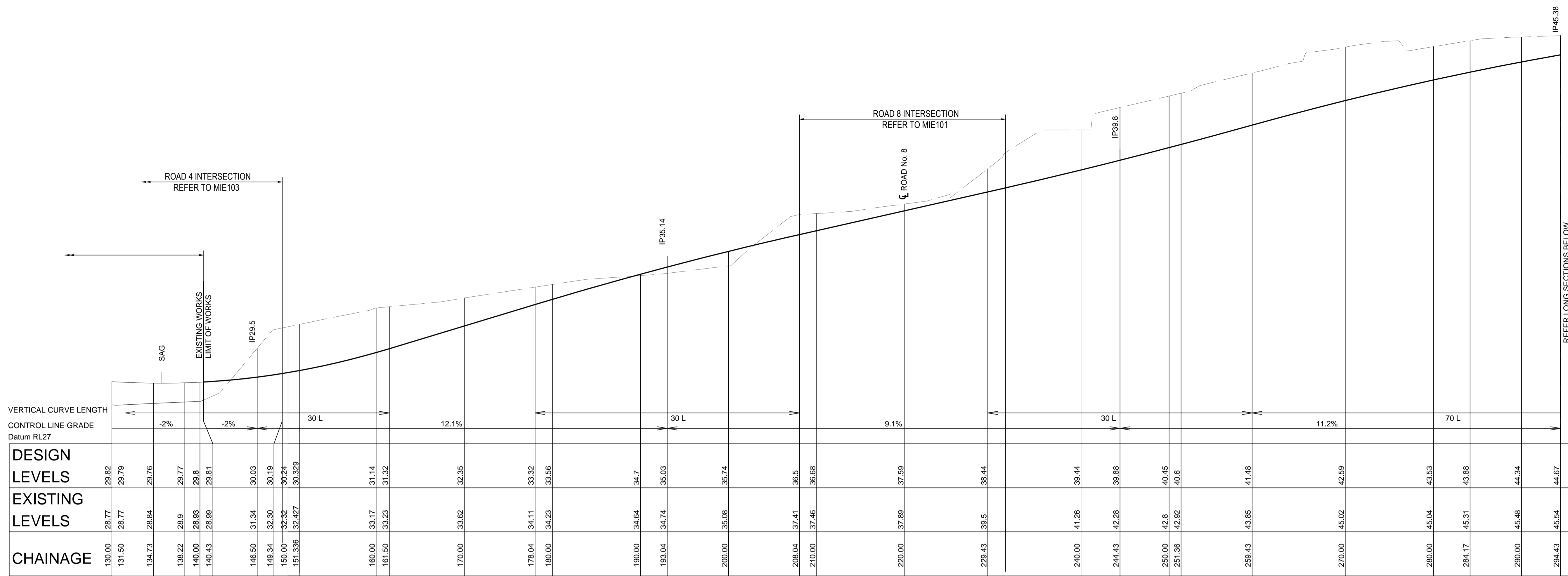
LONGITUDINAL SECTION - ROAD 5 HORIZONTAL SCALE 1:250 VERTICAL SCALE 1:100
