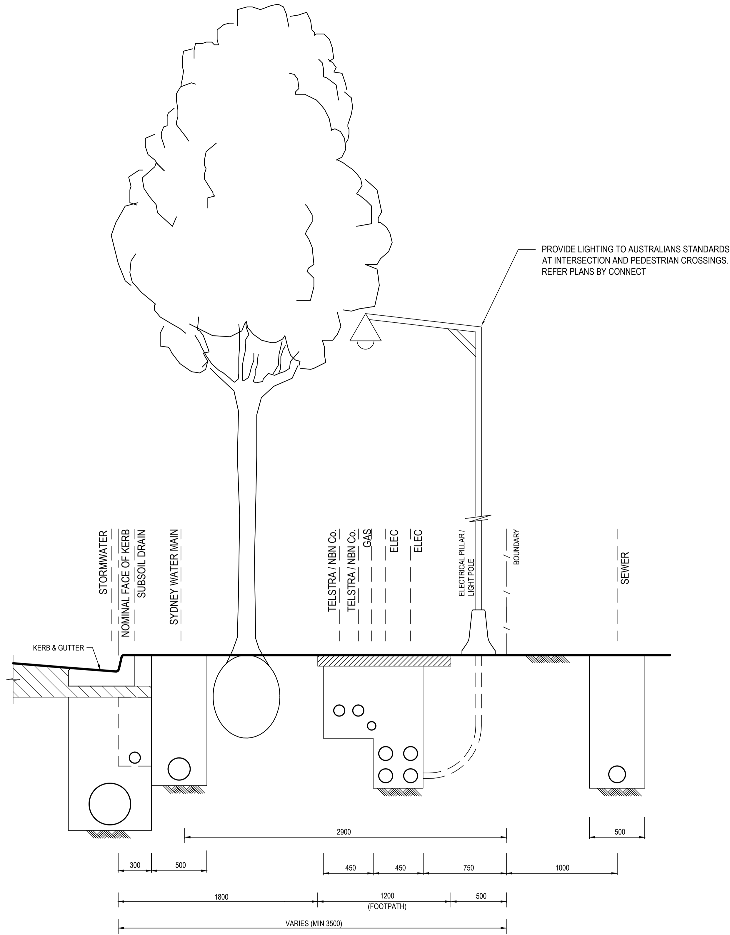
TYPICAL FOOTWAY NOT TO SCALE
