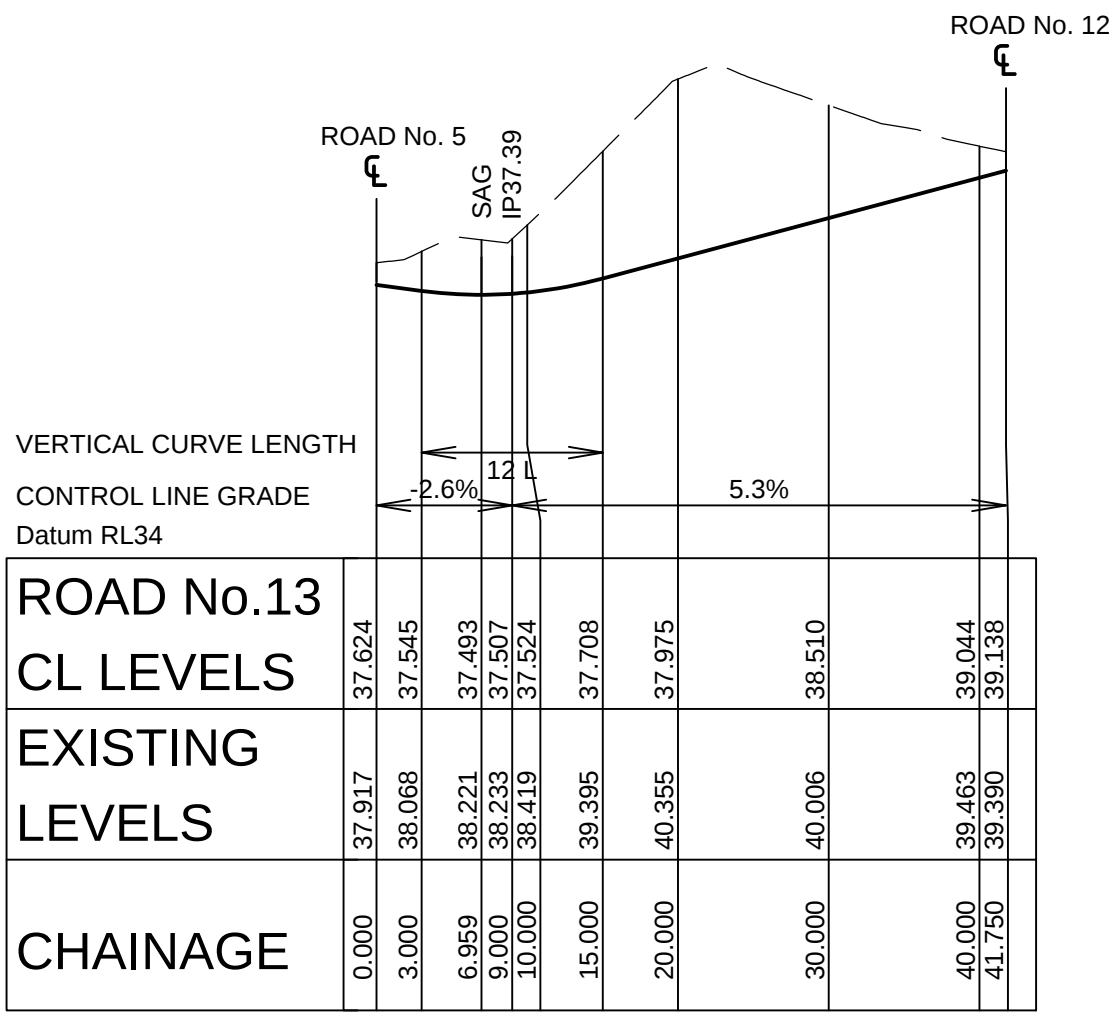
LONGITUDINAL SECTION ROAD No. 13 (PRIVATE ROAD) HORIZONTAL SCALE 1:500 VERTICAL SCALE 1:100
