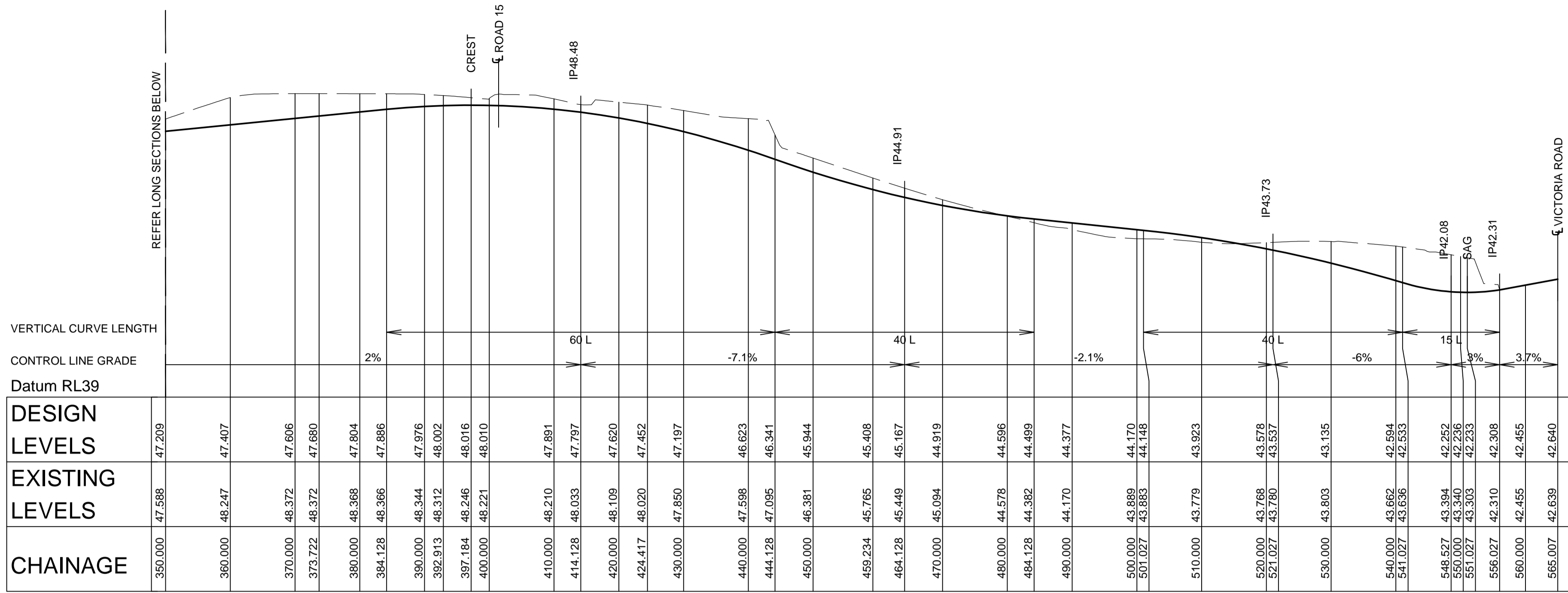
LONGITUDINAL SECTION - ROAD 5 HORIZONTAL SCALE 1:500 VERTICAL SCALE 1:100
