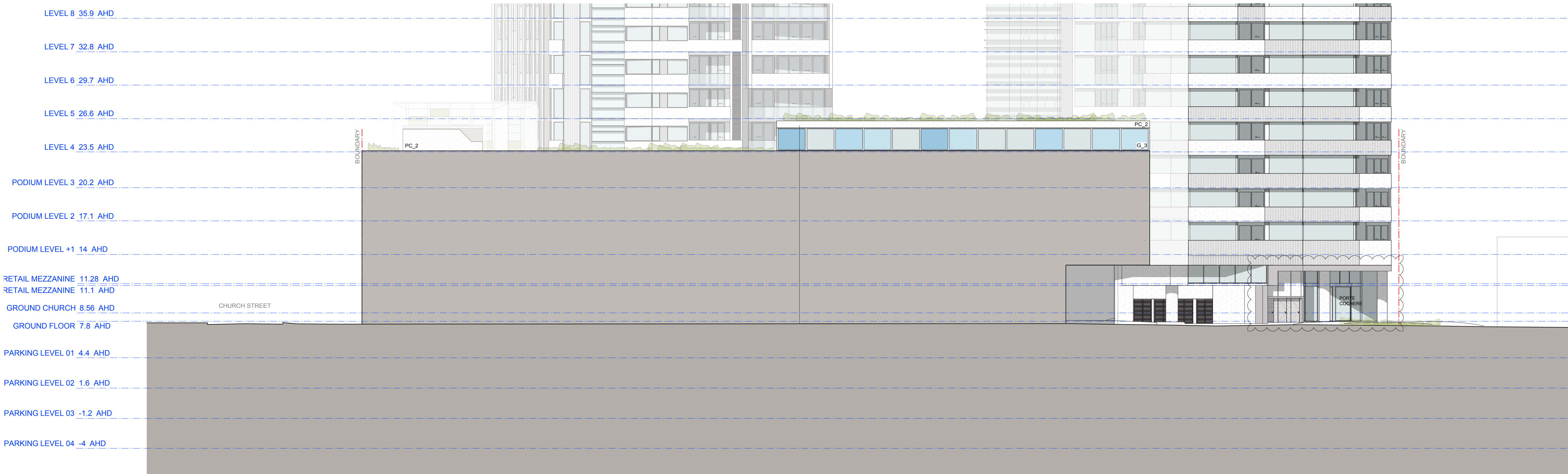
2 ELEVATION - SOUTH 1:200 @A1
