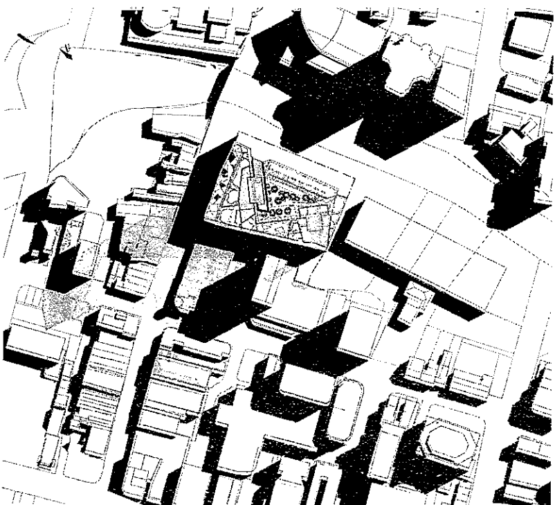
SHADOW DIAGRAM - EQUINOX (MARCH 21ST) 9.00AM 1:2000 @ A1
