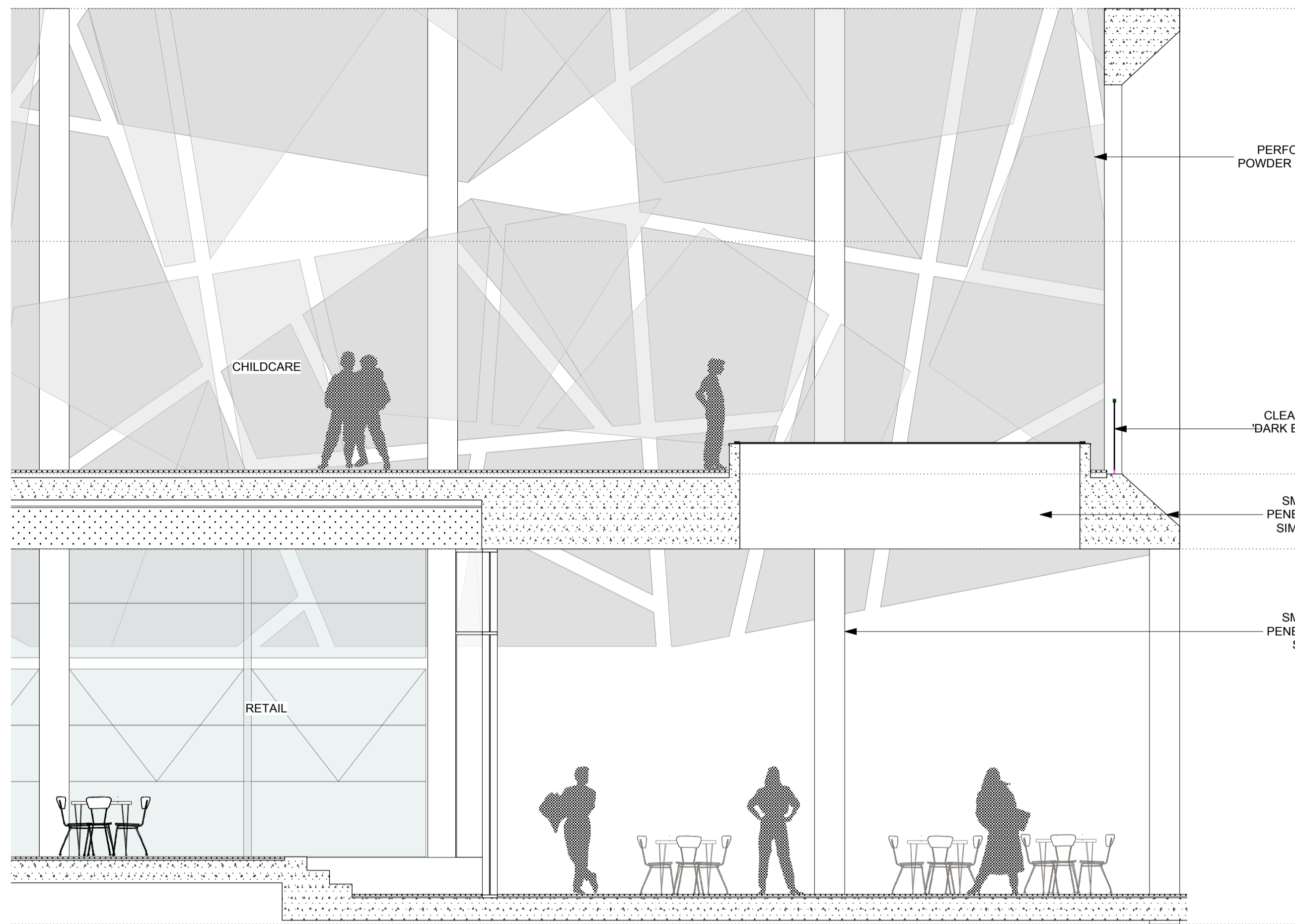
01 DETAIL SECTION 1:50
