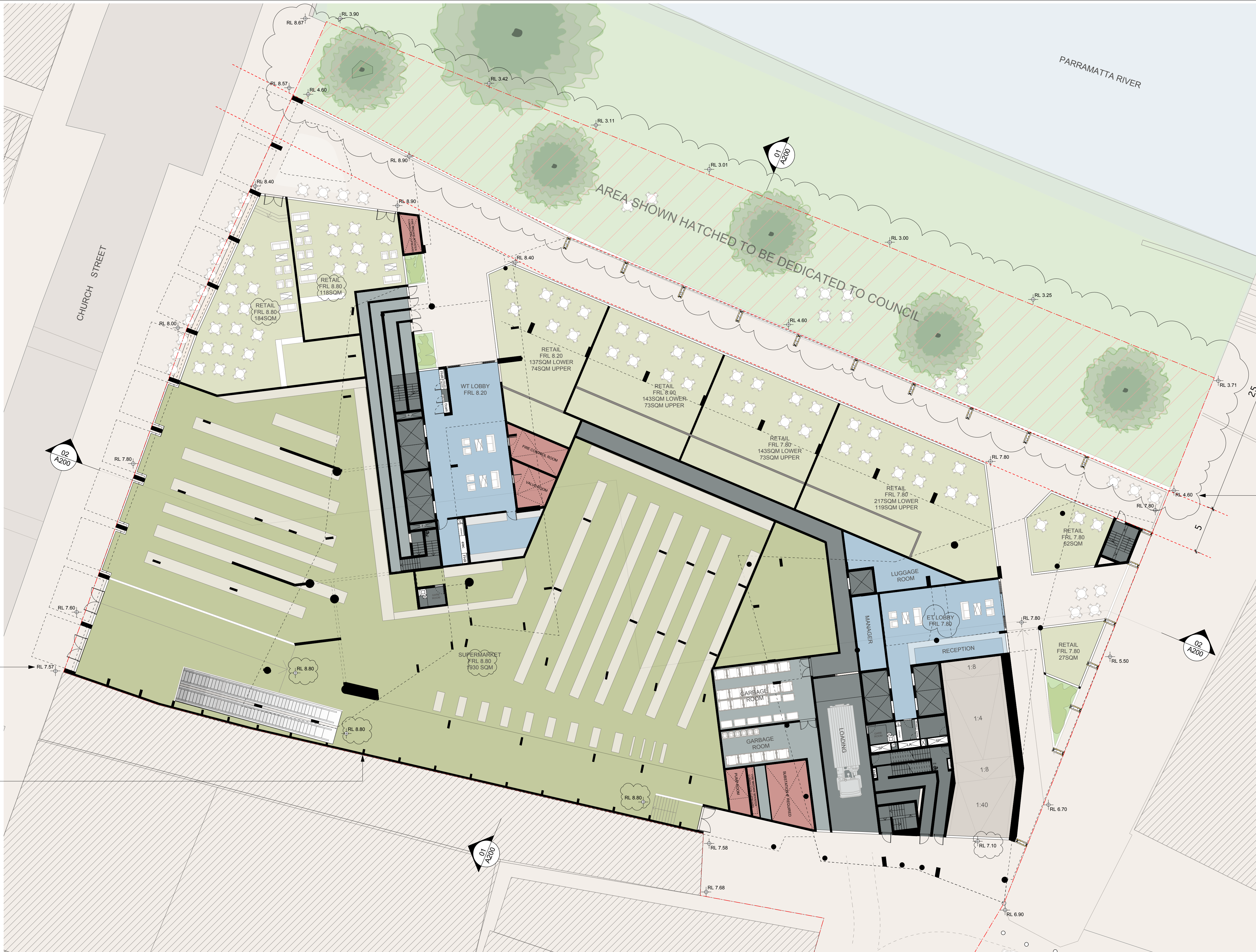
01 PLAN - LEVEL 00 (RETAIL) 1:200 @ A1
