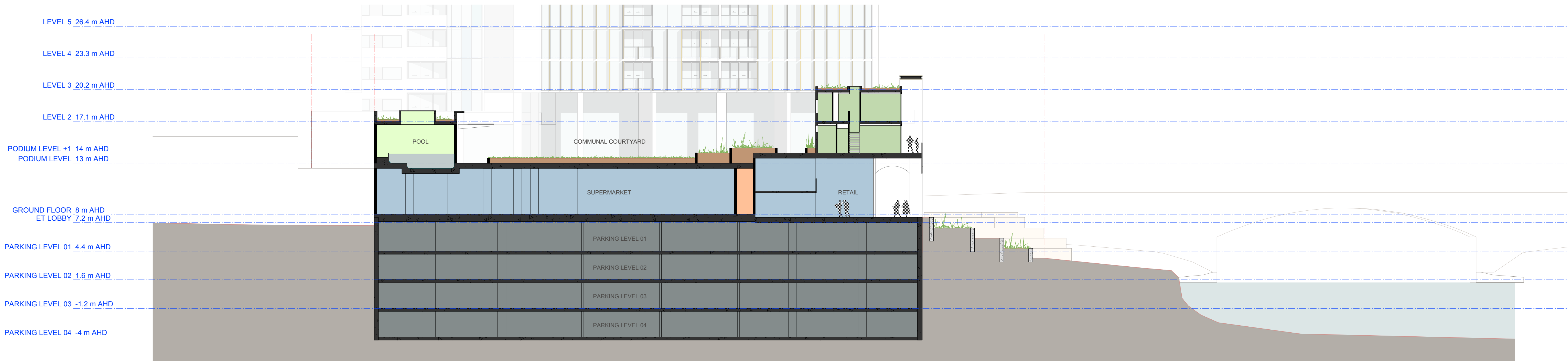
01 SHORT SECTION LOOKING WEST 1:200 @A1
