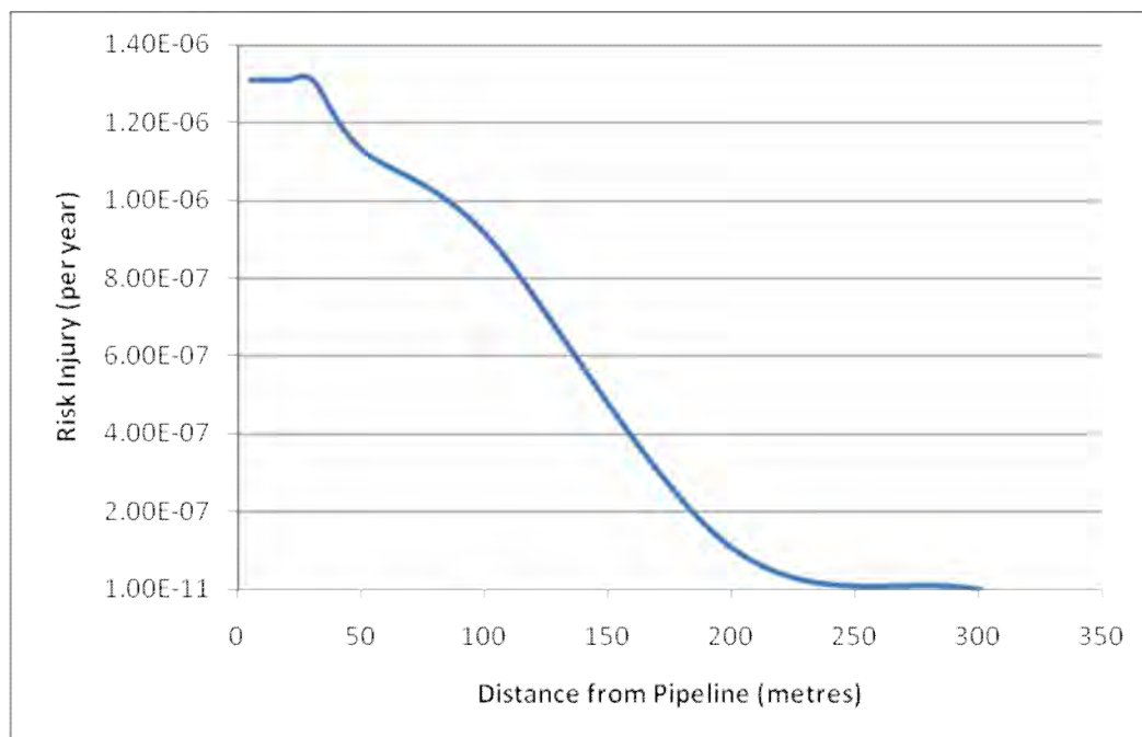
Figure 5 – Injury Risk Transects for the 6.8MM Gas Pipeline
