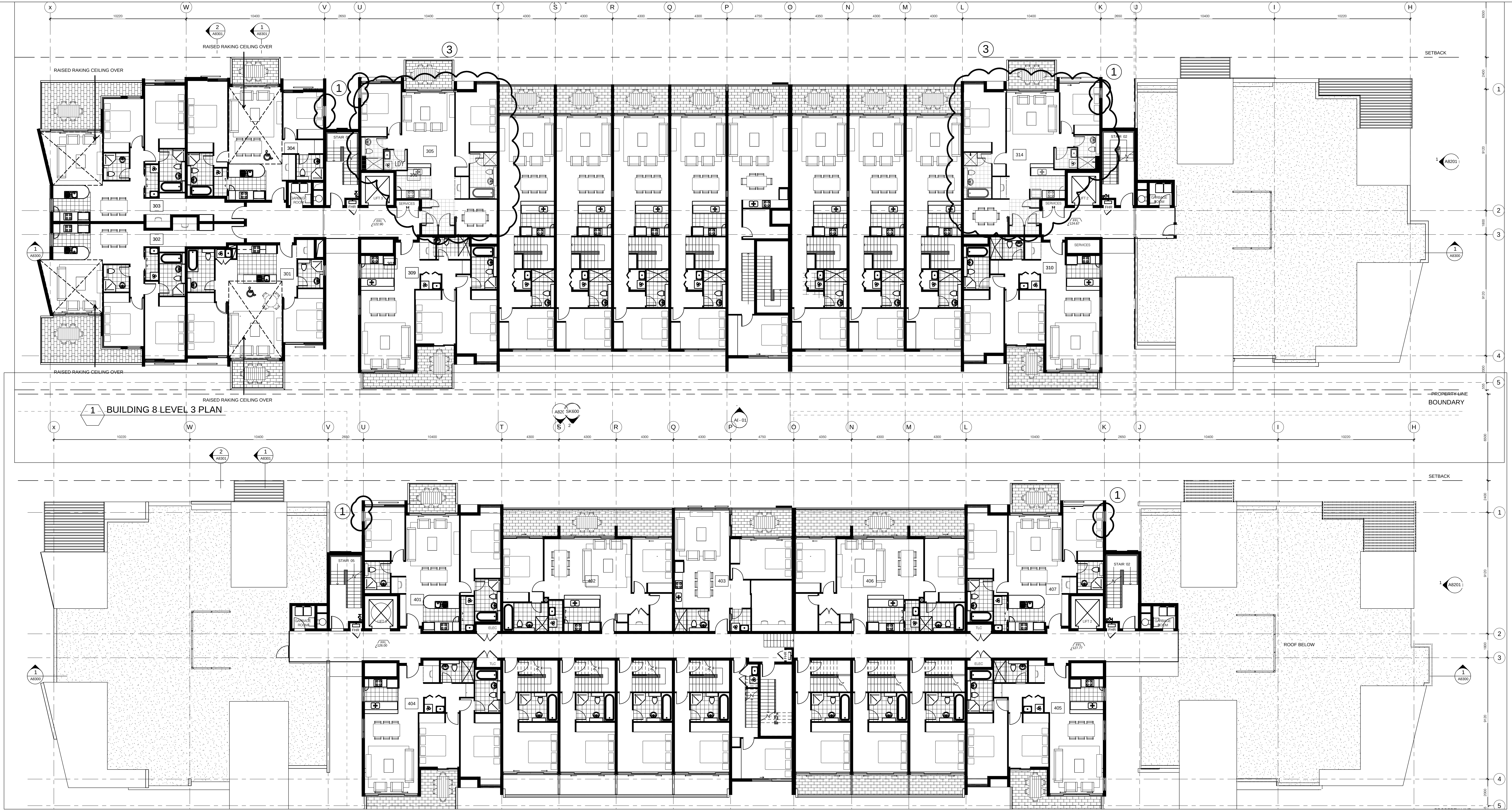
2 BUILDING 8 LEVEL 4 PLAN
