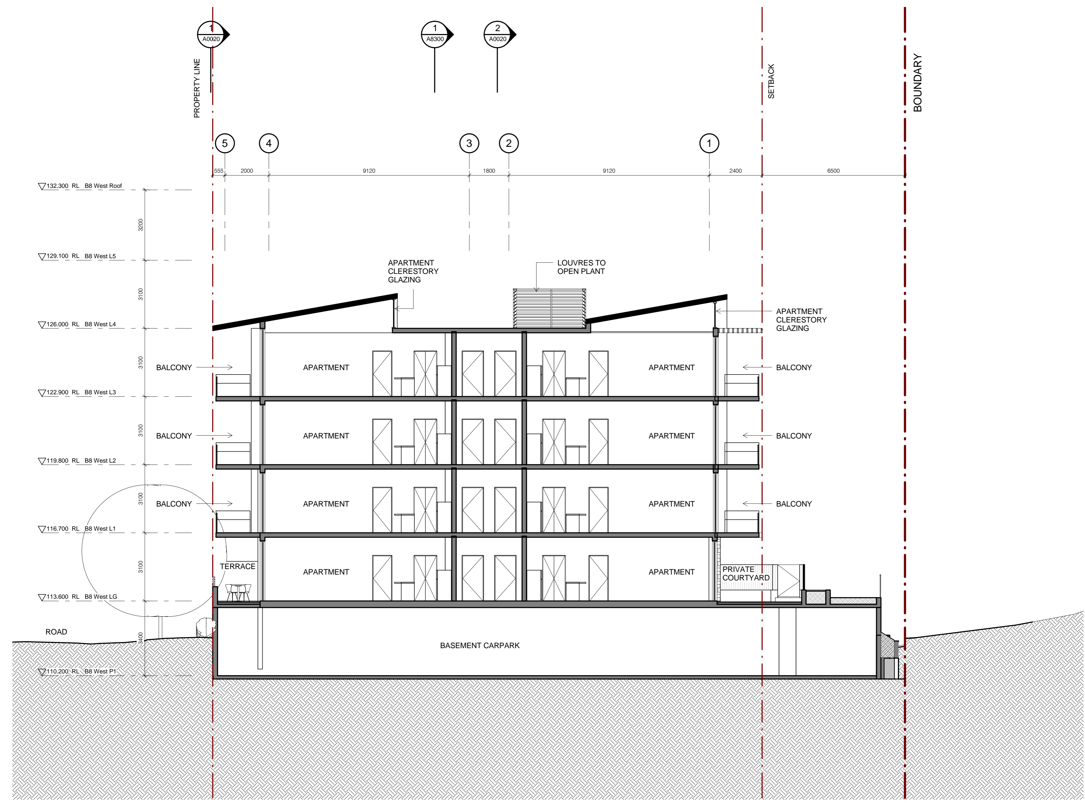
1 SECTION E - BUILDING 8 1 : 100
