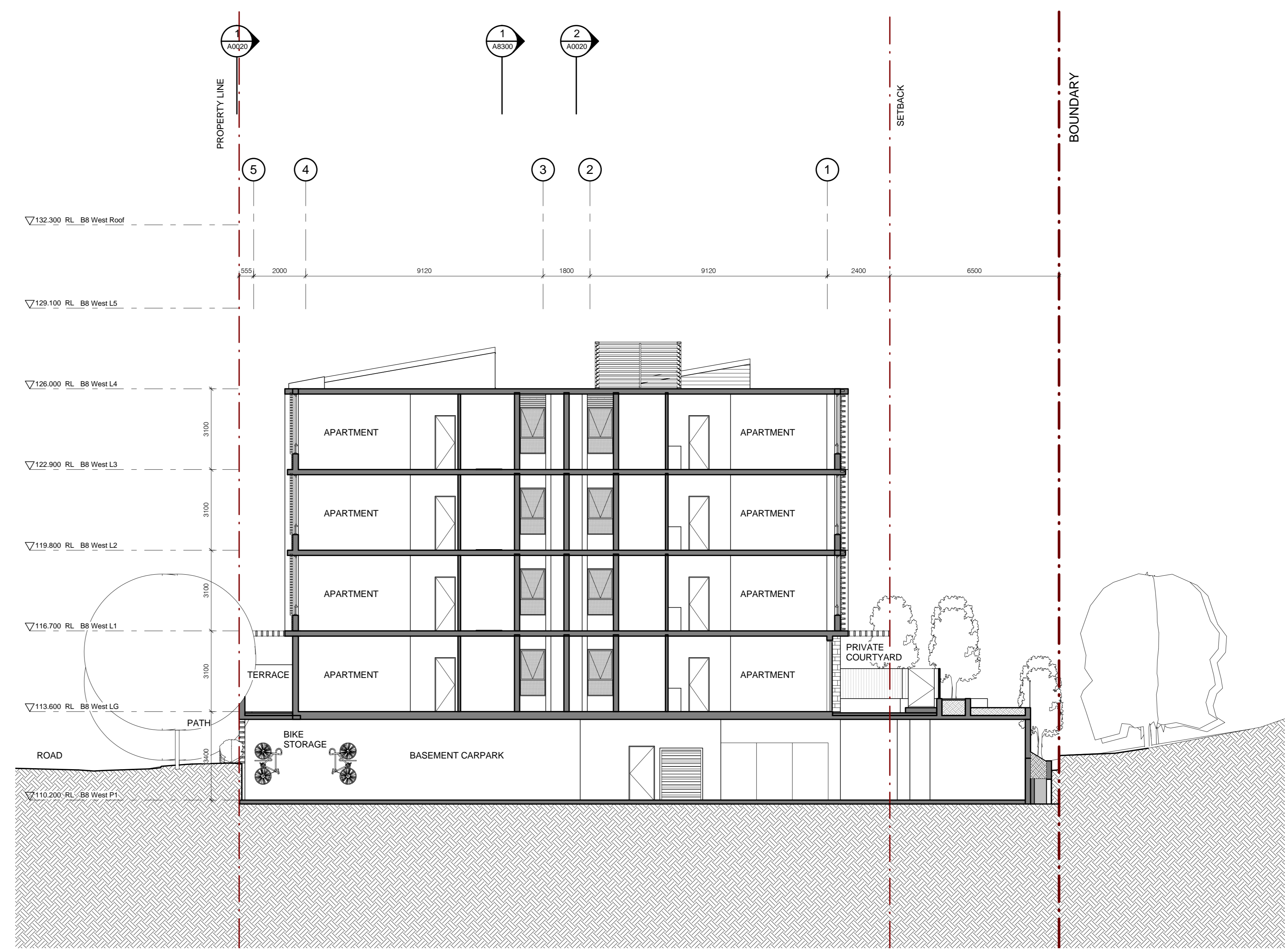
2 SECTION F - BUILDING 8 1 : 100
