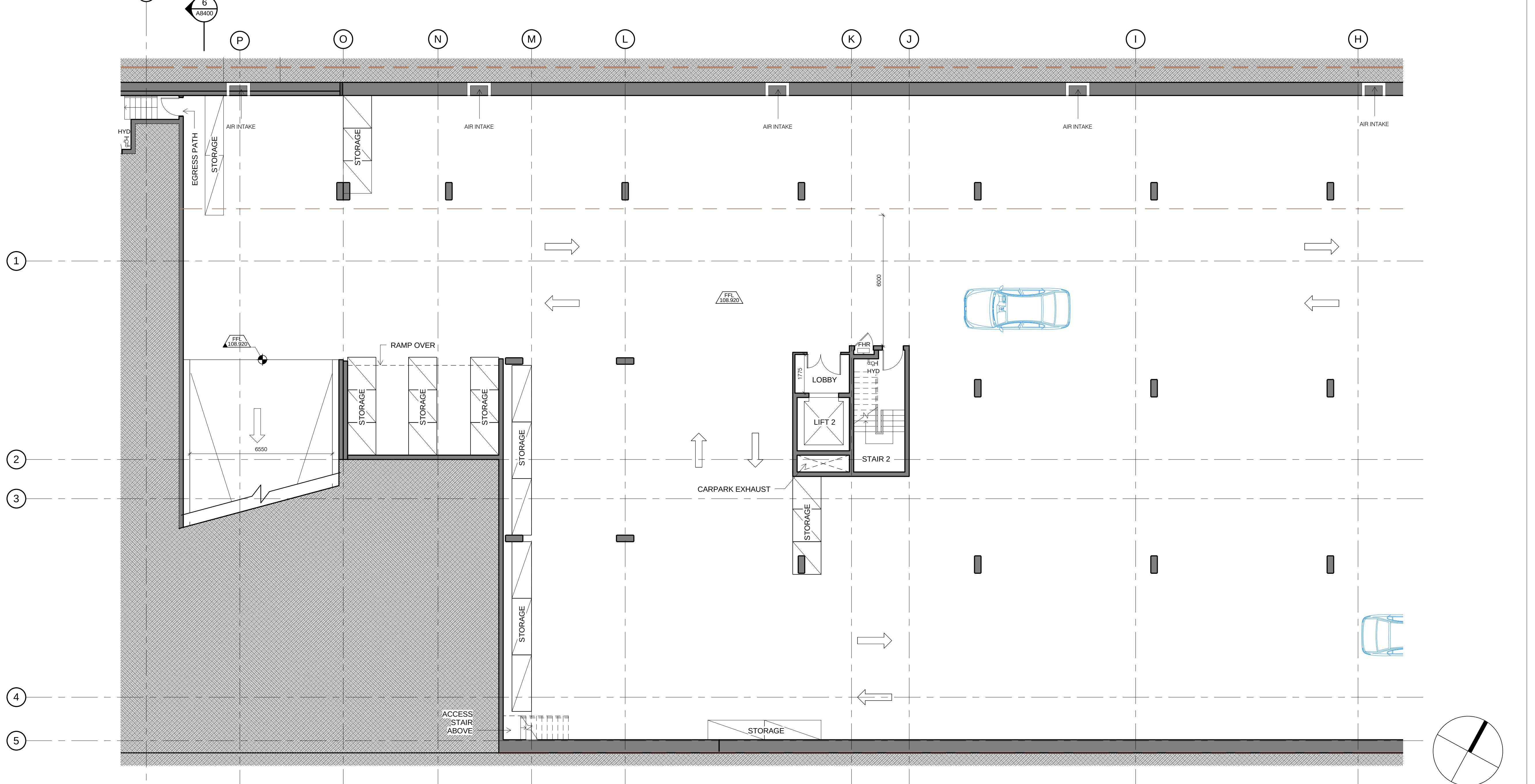
3 BUILDING 8 LEVEL P2 PLAN 1 : 100
