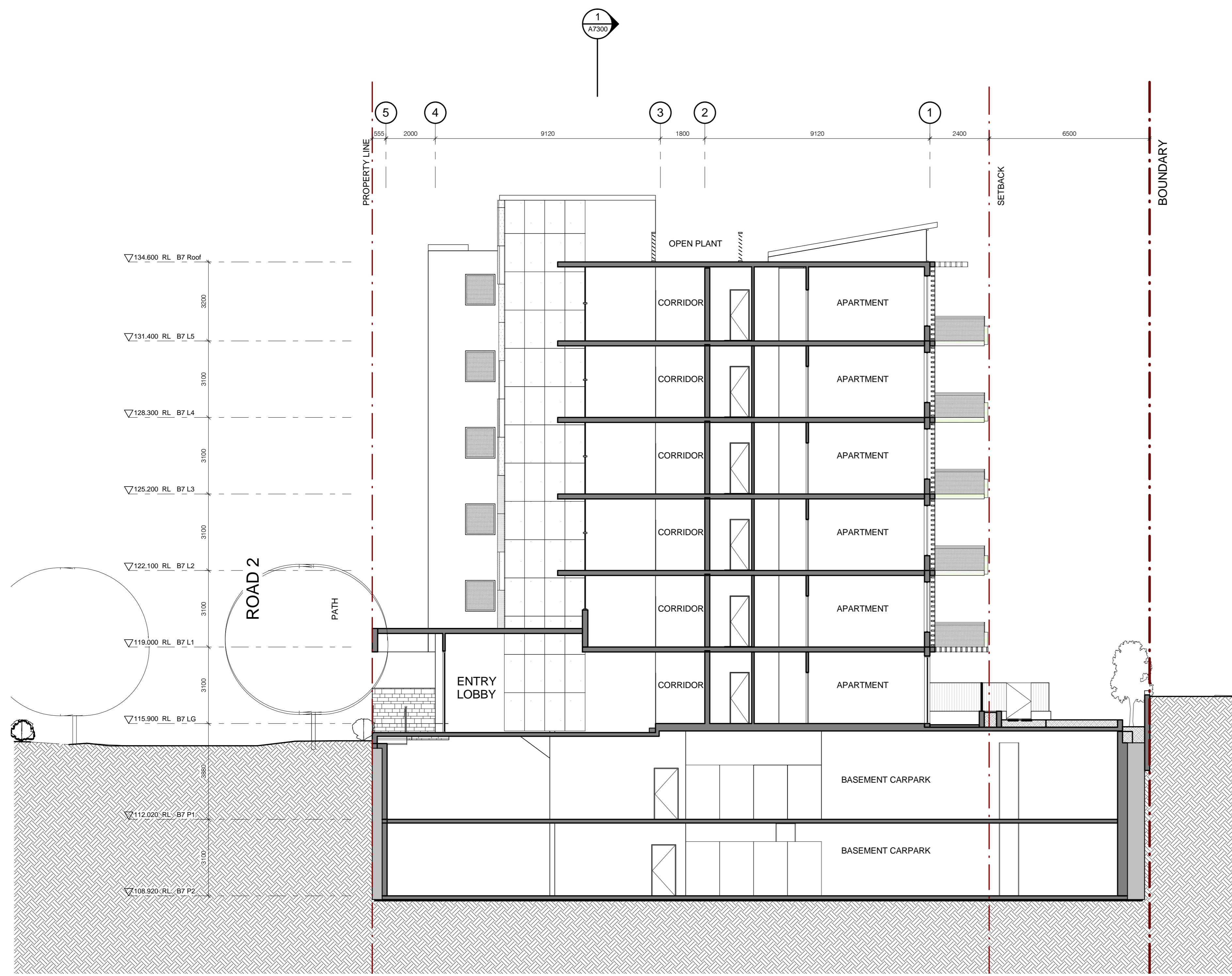
1 SECTION B - BUILDING 7 1 : 100
