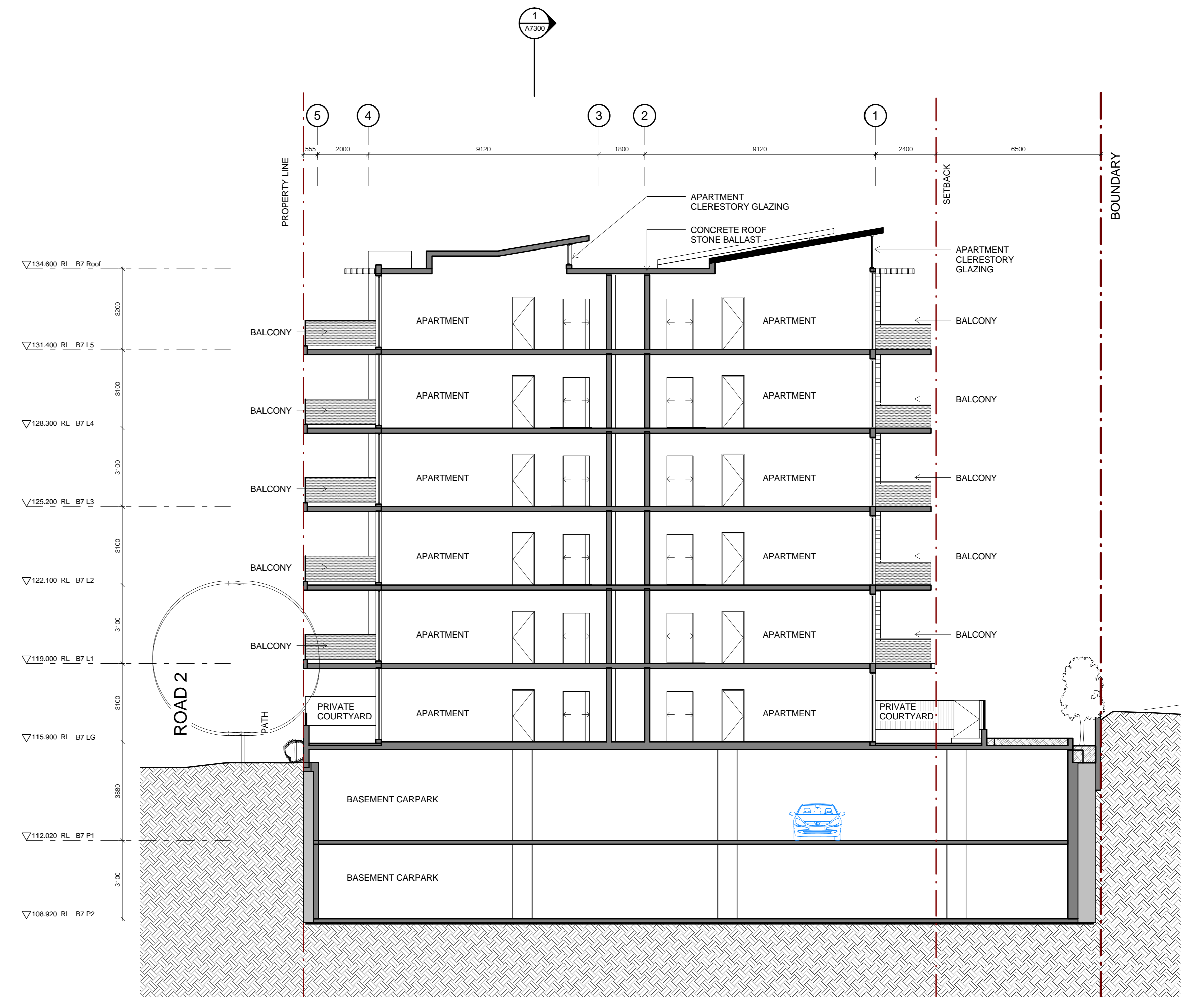
2 SECTION C - BUILDING 7 1 : 100
