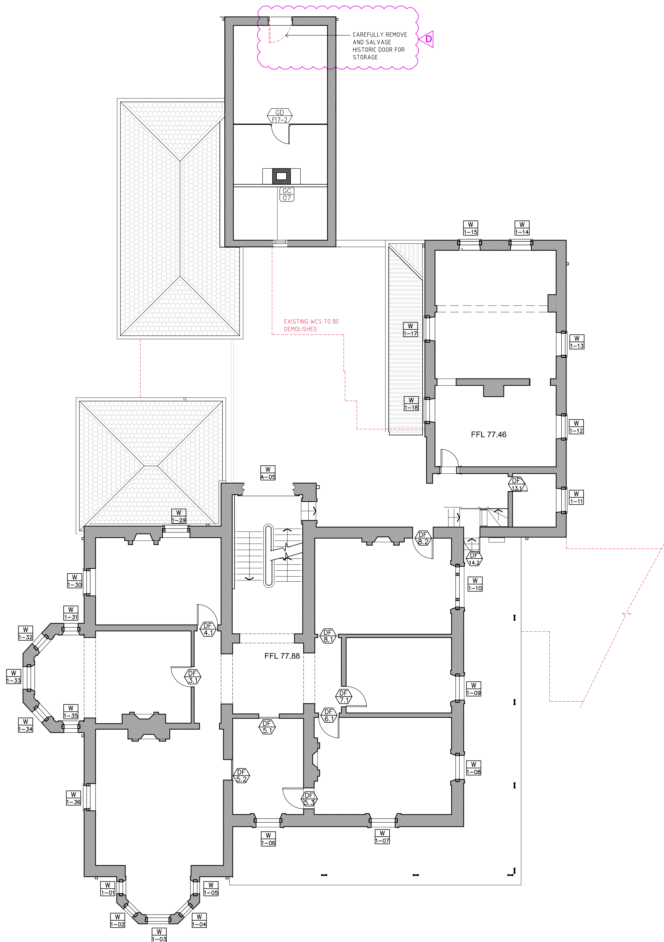
02 FIRST FLOOR DEMOLITION PLAN 1:100
