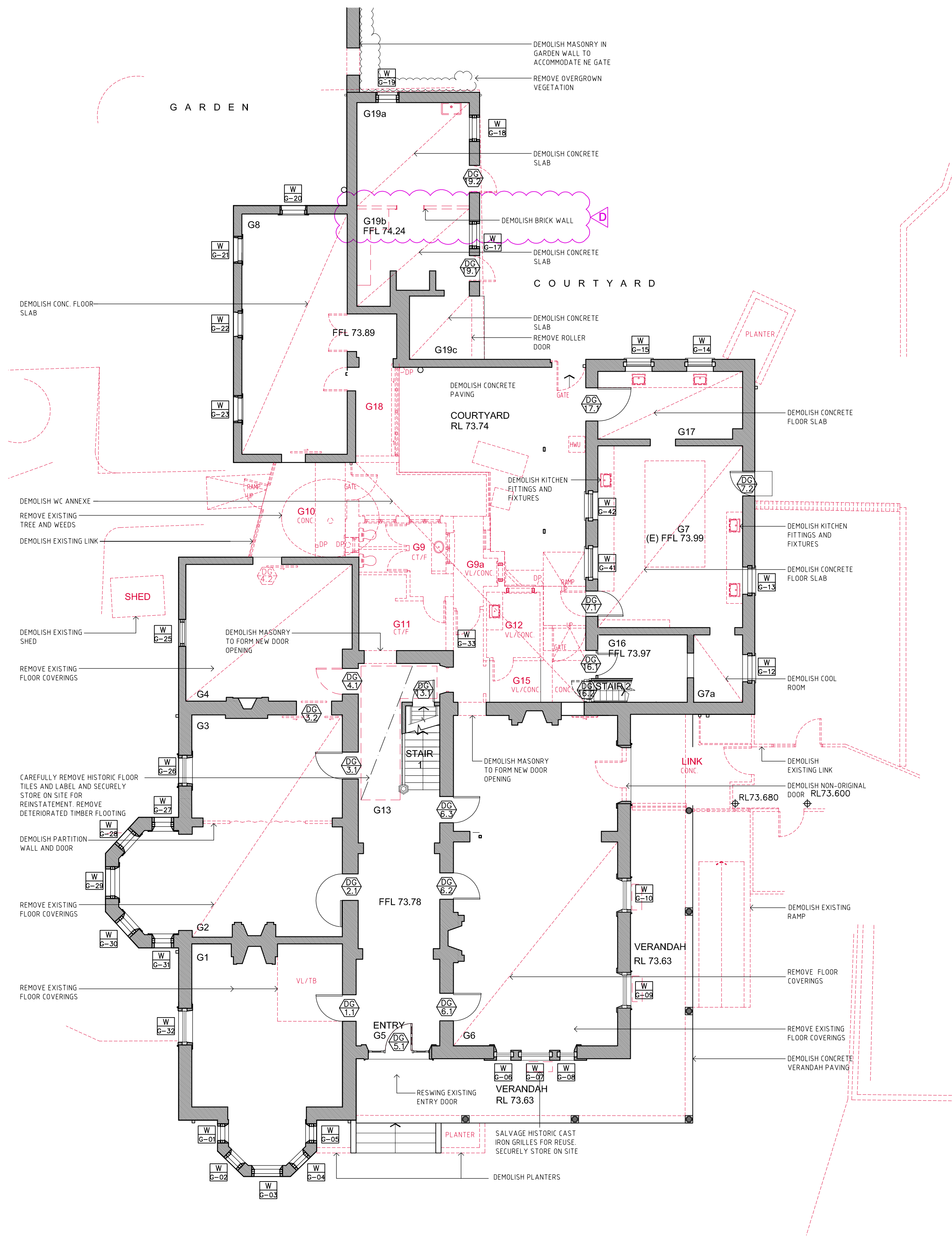
01 GROUND FLOOR DEMOLITION PLAN 1:100
