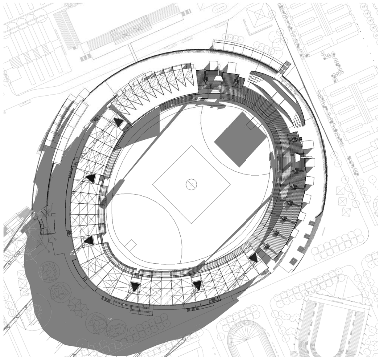
3 Stage 1A Shadow - 21st Jun 9am
