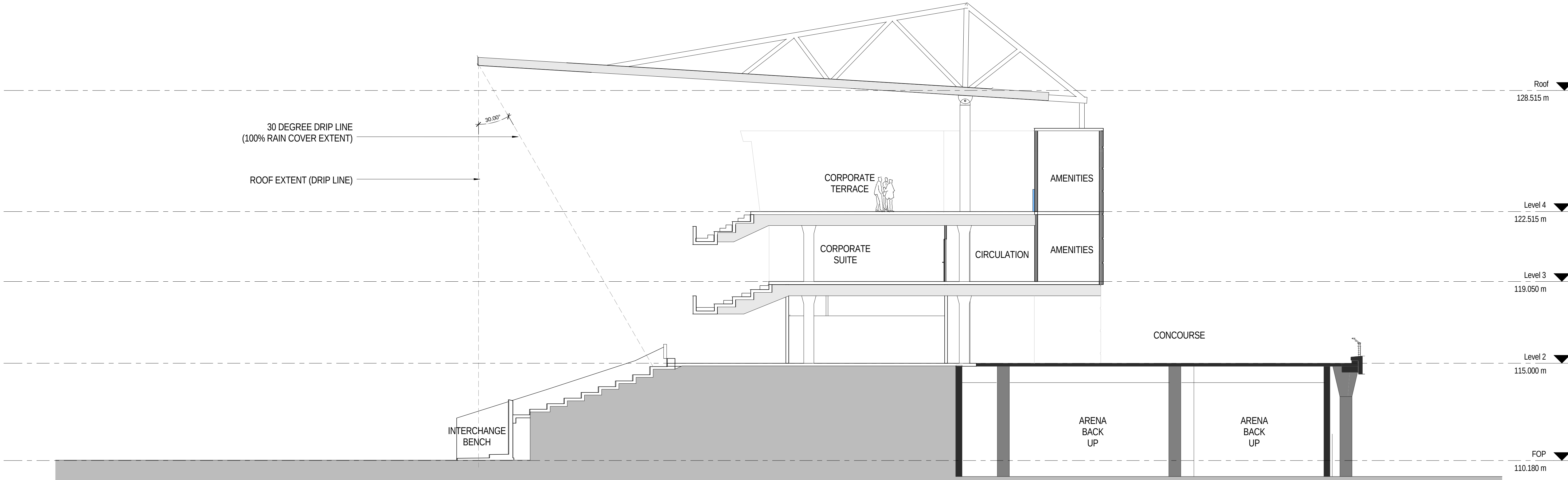
2 Stage 1a - NE Section Typical - Grid B7 1 : 100
