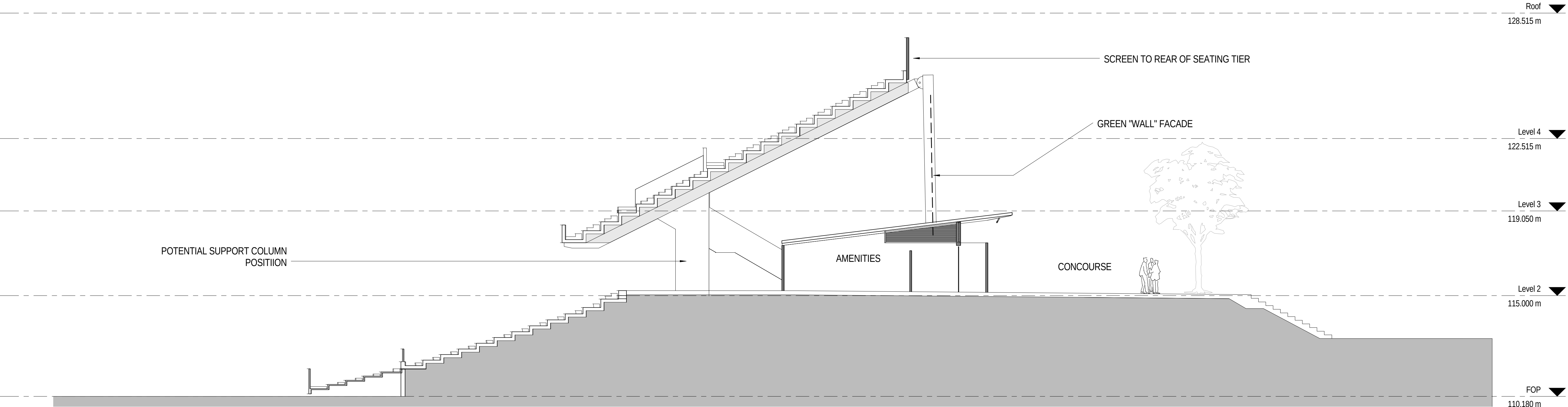
1 Stage 1a - SE Section Typical - Grid B40 1 : 100
