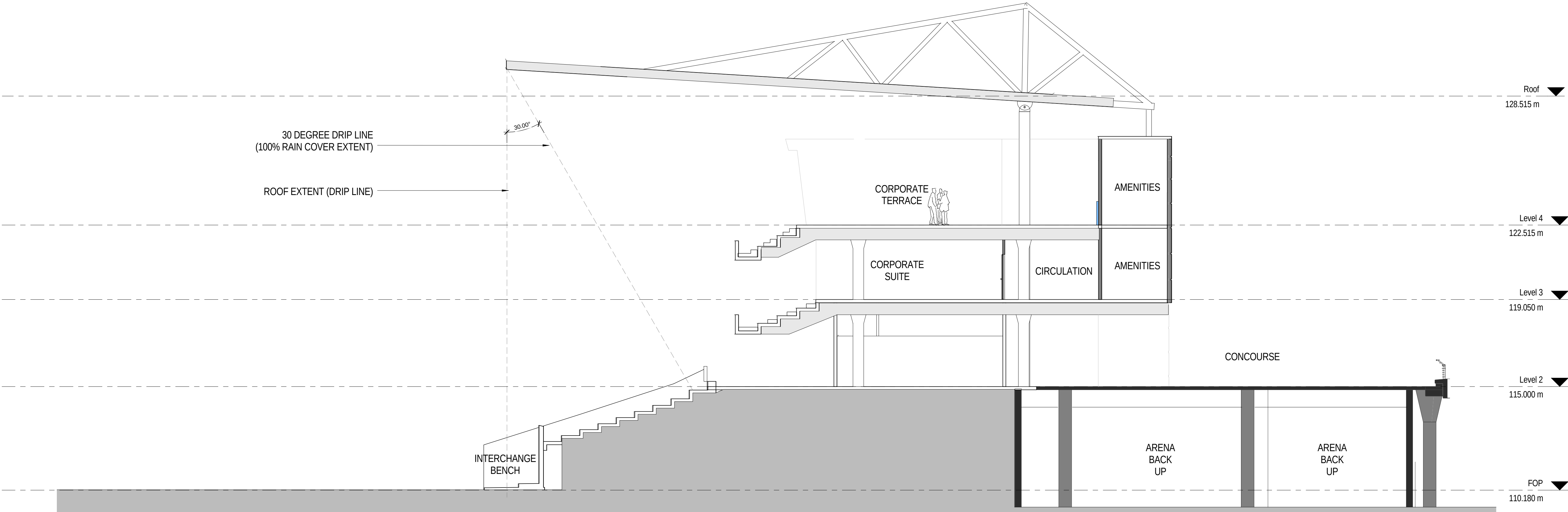
2 Stage 1 - NE Section Typical - Grid B7 1 : 100
