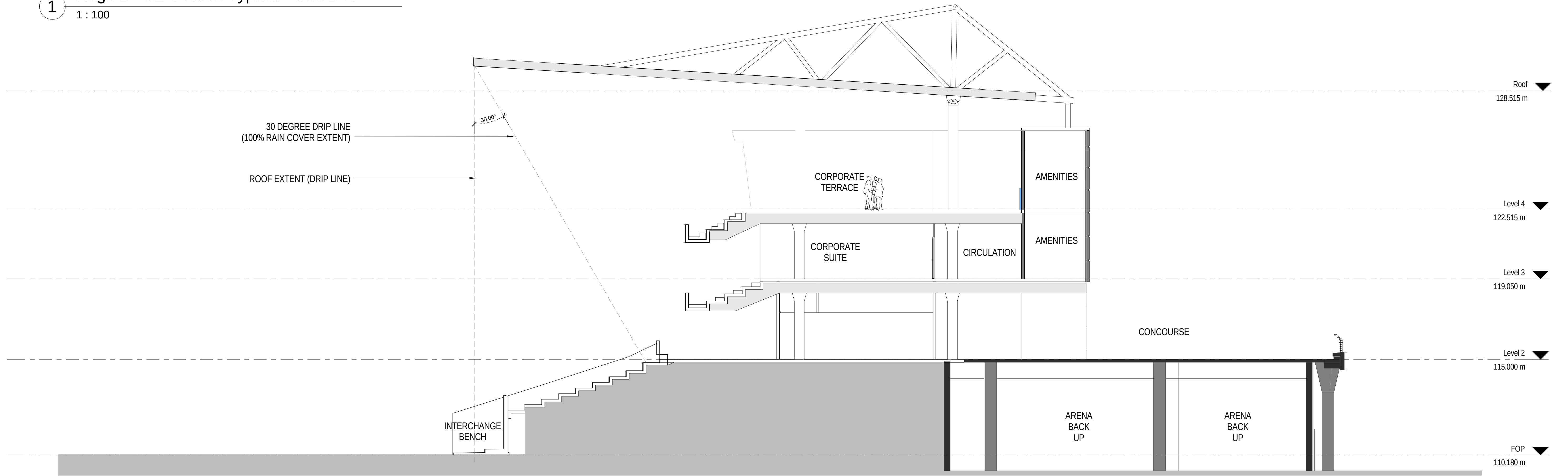
2 Stage 2 - NE Section Typical - Grid B7 1 : 100
