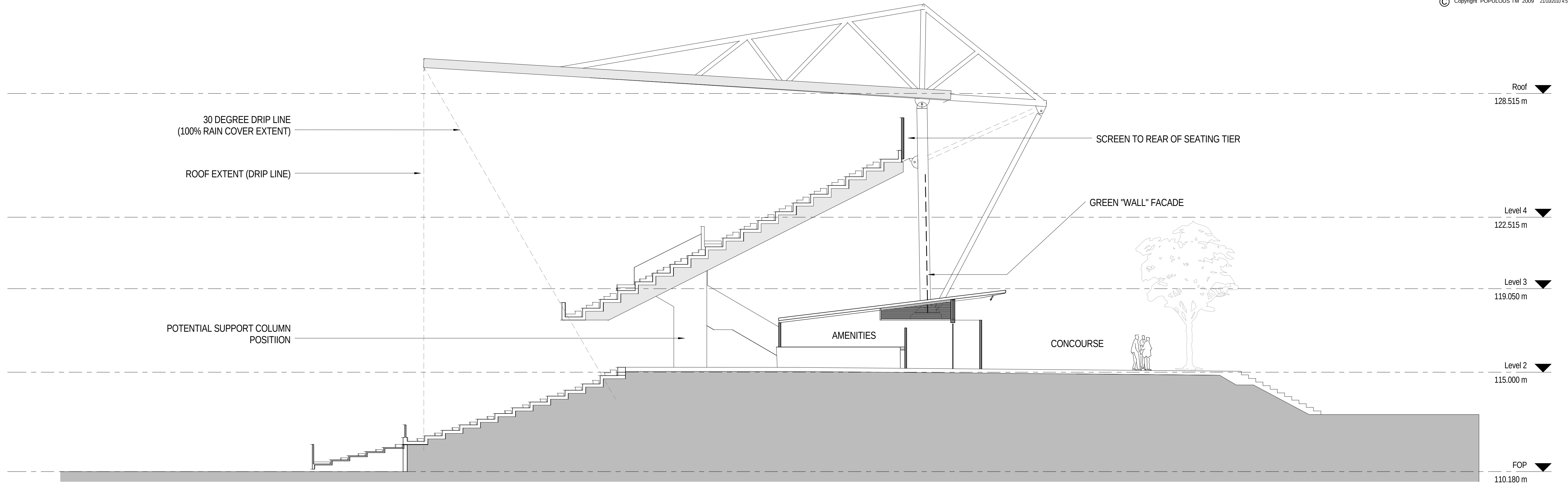
1 Stage 2 - SE Section Typical - Grid B40 1 : 100
