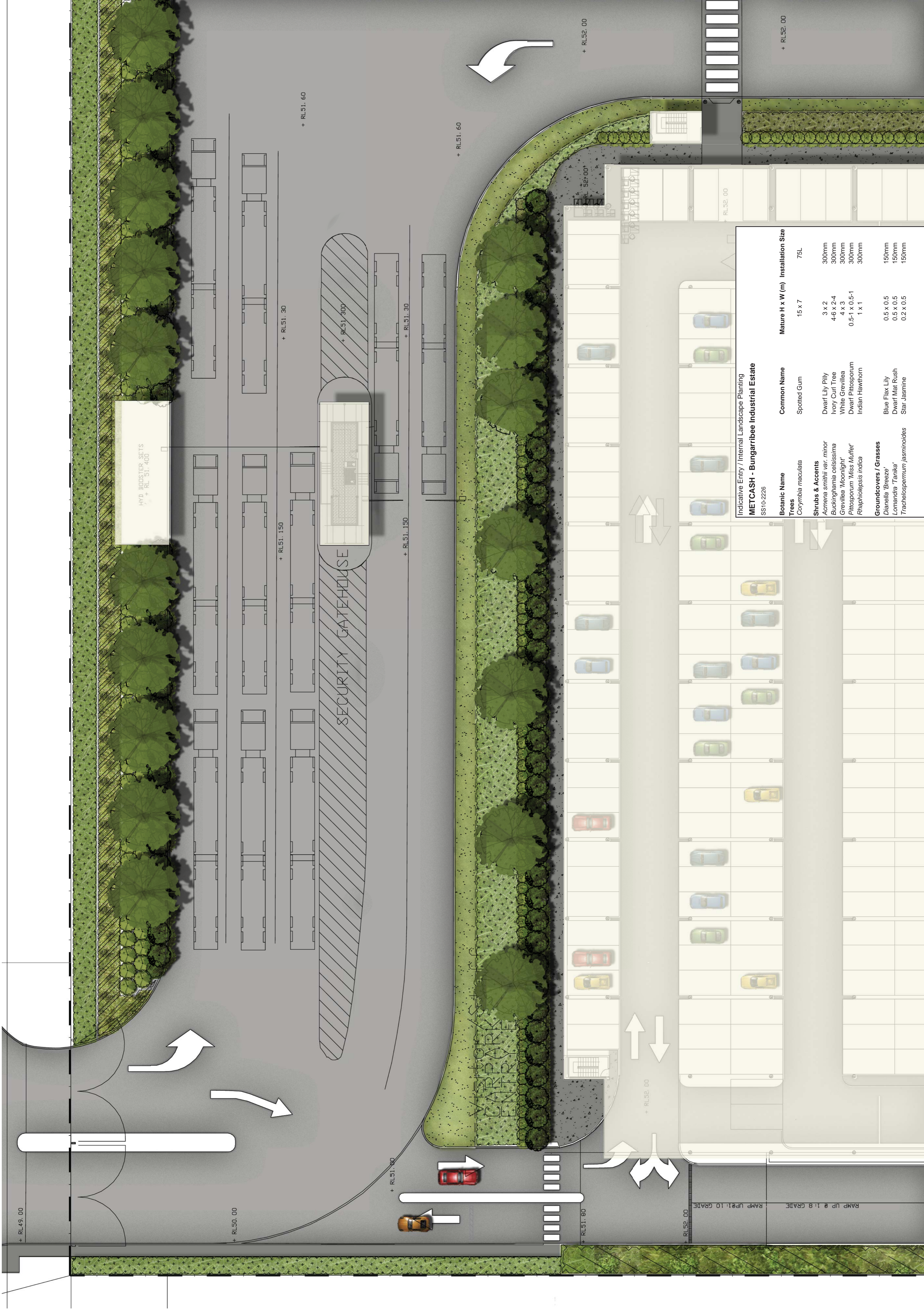
1. PRESENTATION / ENTRY LANDSCAPE SCALE 1:200
