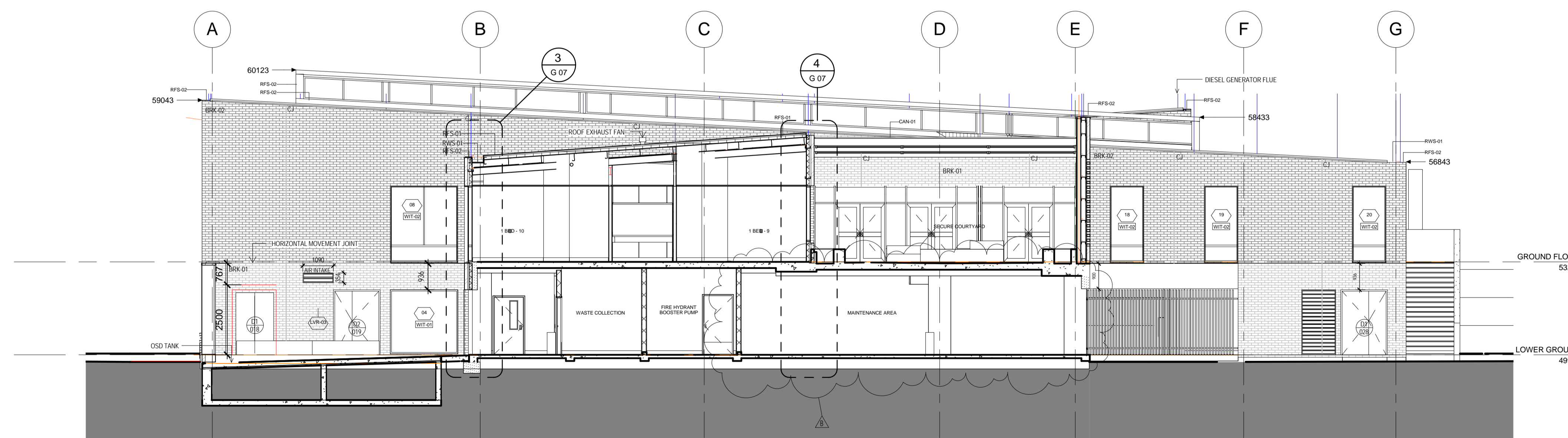
3 SECTION GRID 6-7 F 03 1:100
