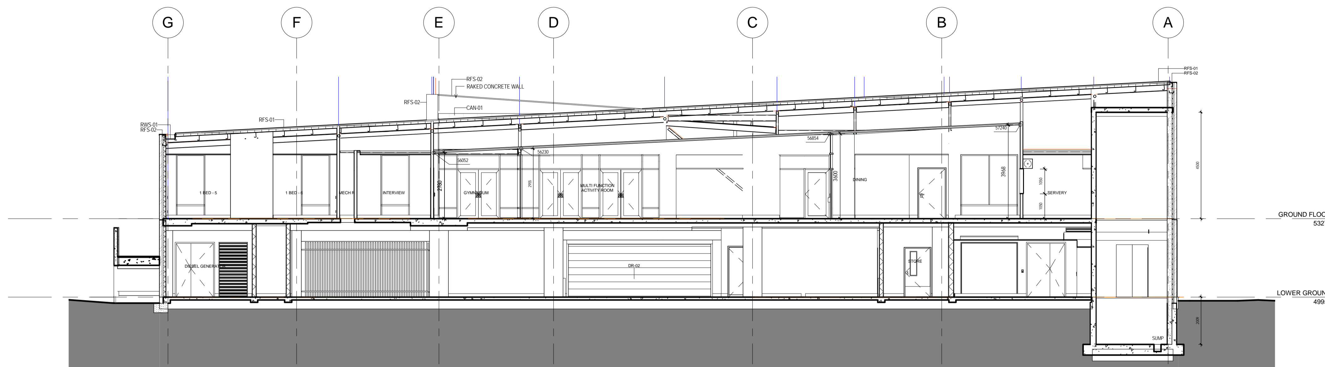
1 SECTION GRID 05 EAST F 03 1:100
