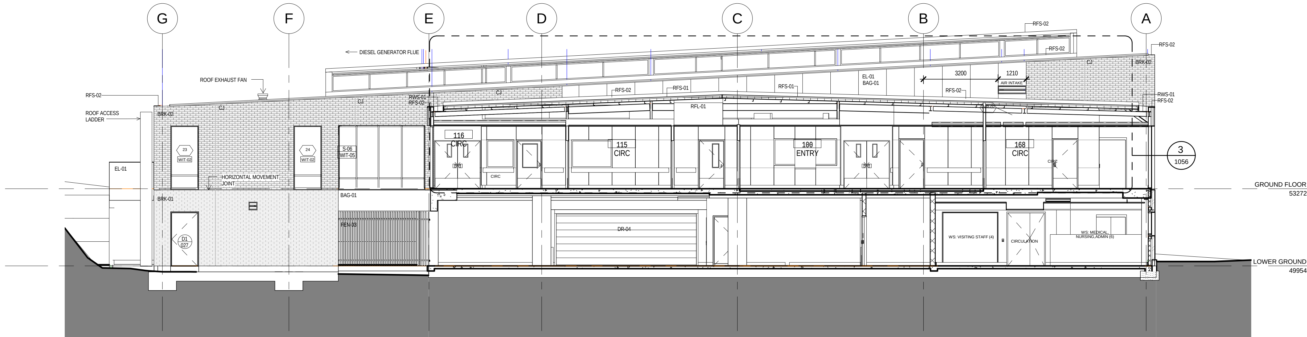
1 SECTION GRID 3-4 EAST F 02 1:100
