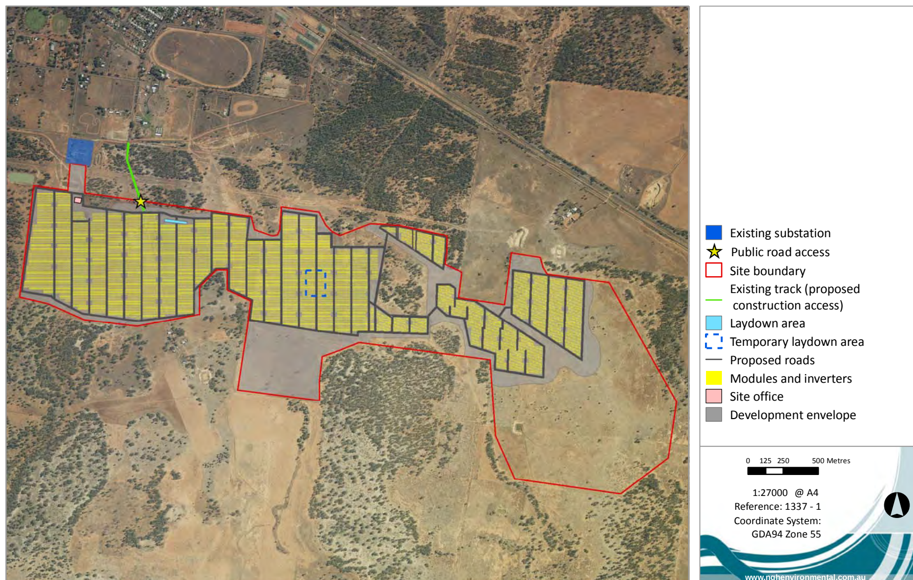
Figure 1-2 Indicative Nyngan Solar Farm layout showing roads, modules and inverters, lay-down areas and site office with the development envelope
