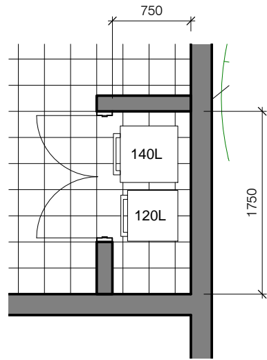
1 BIN STORE BLDG 1 PARKING PLAN (TYPE 1) 1 : 50
