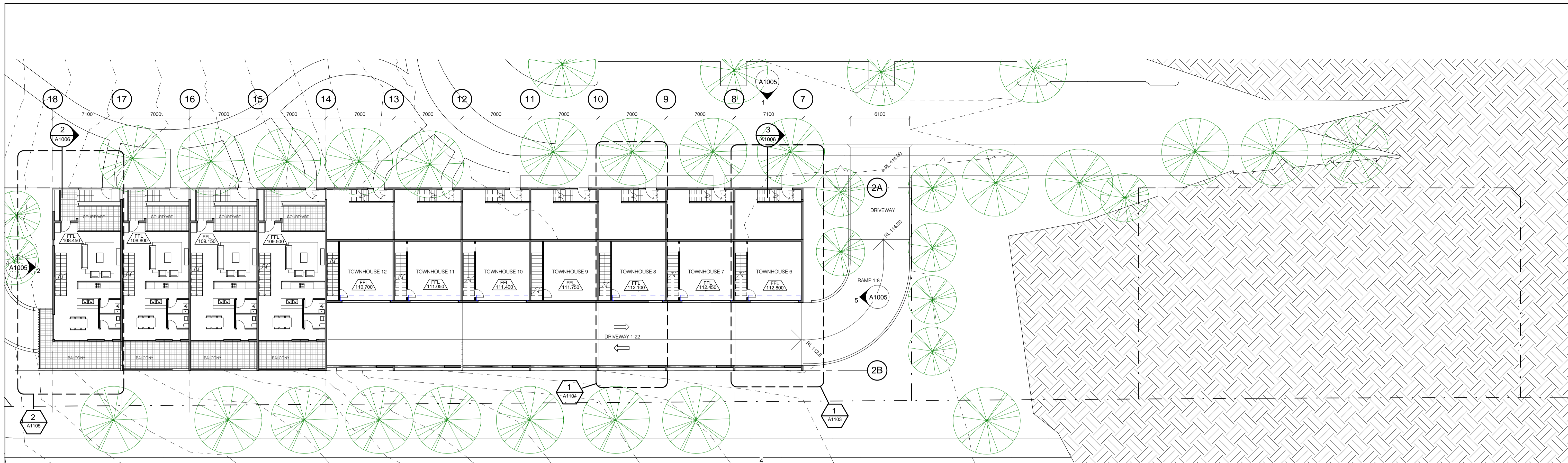
2 BLDG 2 PARKING LEVEL PLAN 1 : 200
