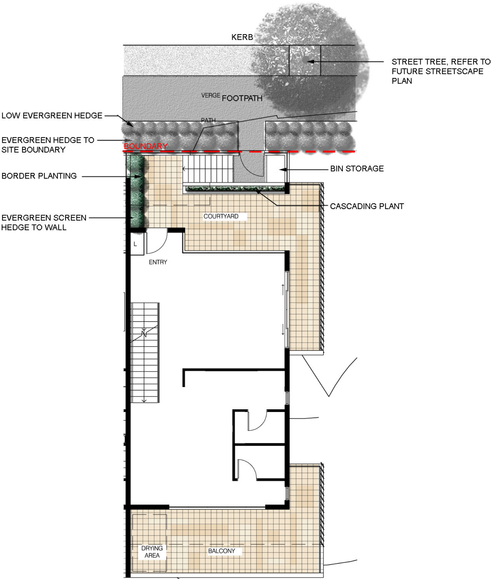
PLAN SCALE 1:200
