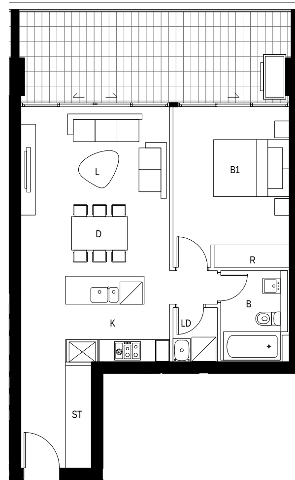
12 DETAIL PLAN BLDG A - Apartment Type 12 1 BED - 55sqm Storage - 5cm
