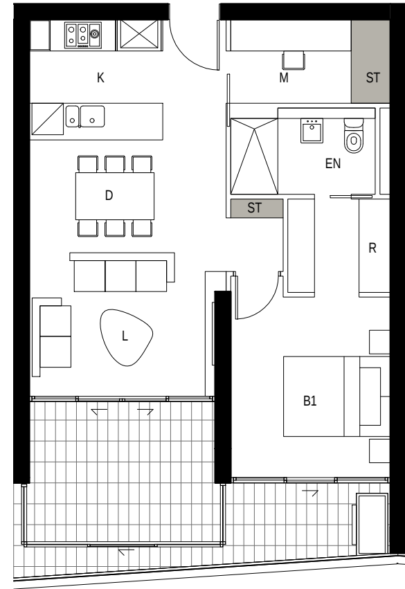
3 DETAIL PLAN BLDG A - Apartment Type 9 1 BED - 54sqm Storage - 3.5cm
