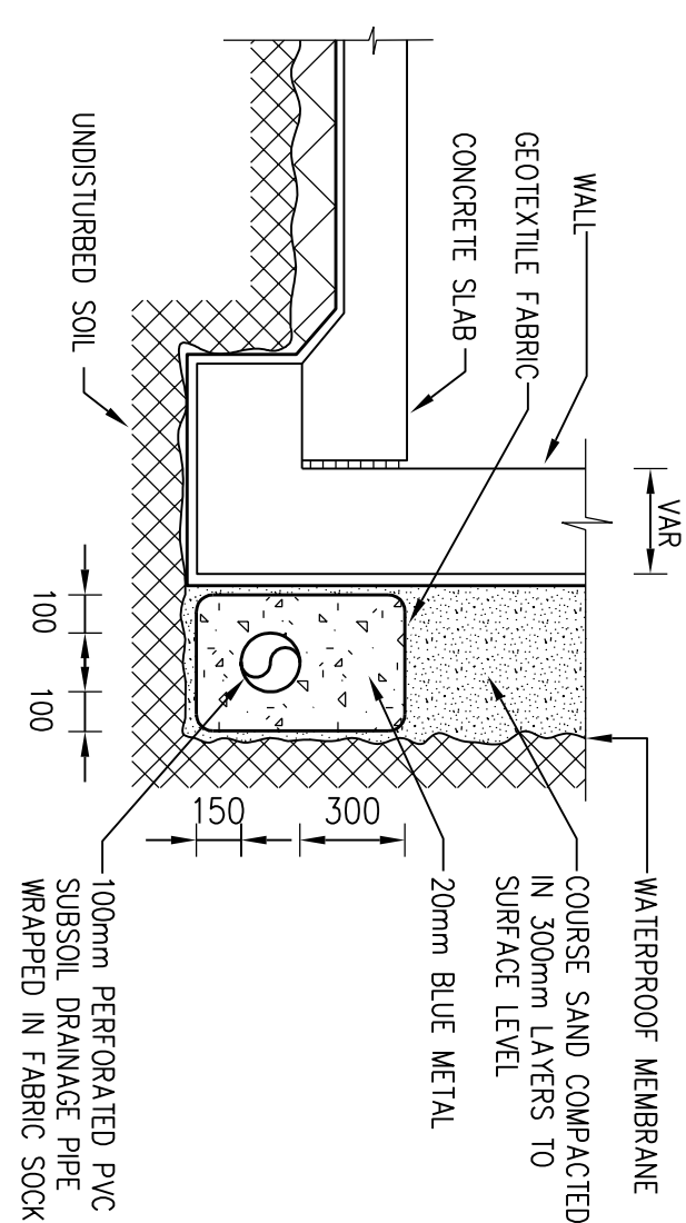
SUBSOIL DRAINAGE SCALE: 1:20
