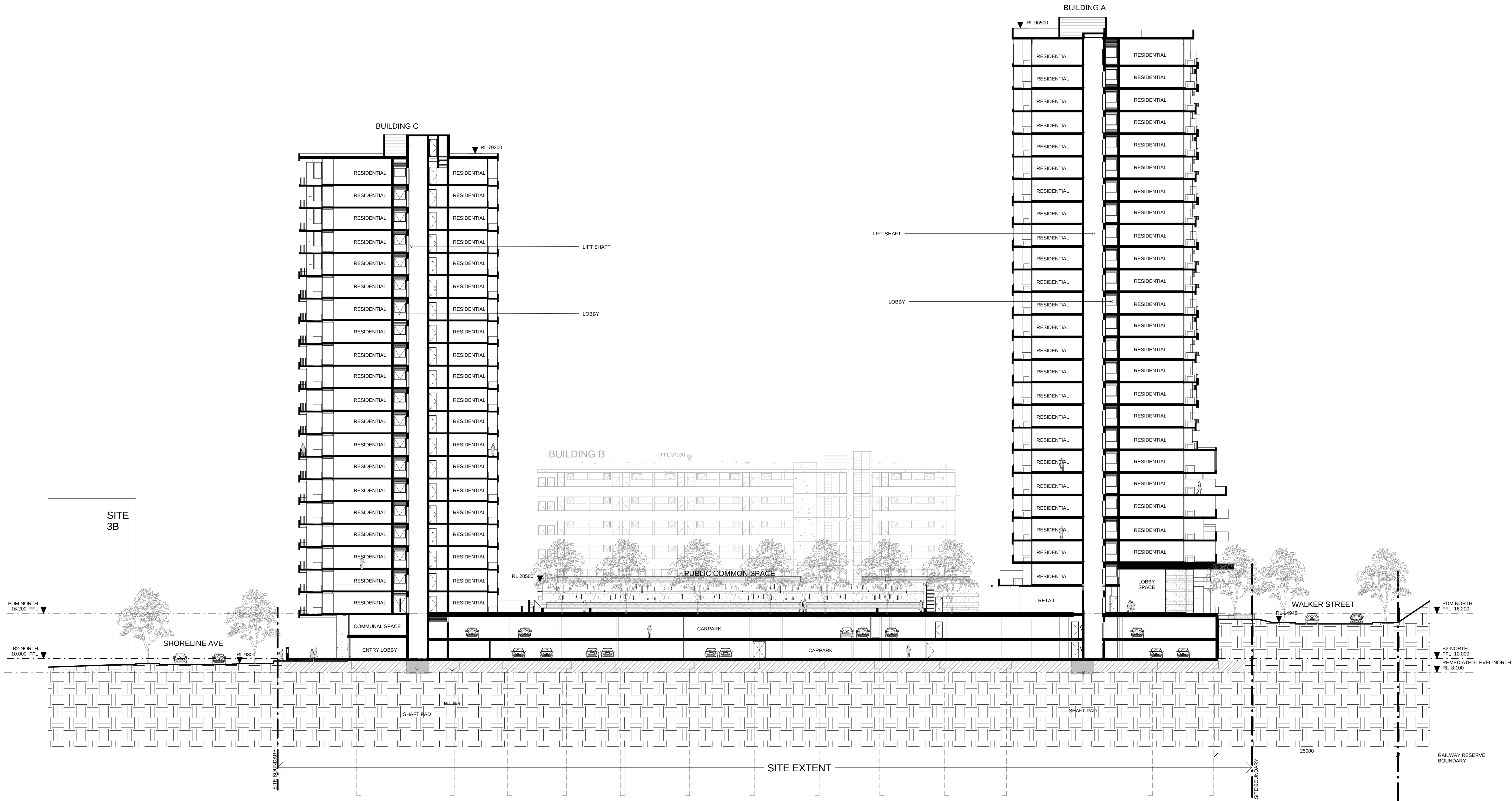
1 SECTION A-5001 East-West Site Section 1 : 250
