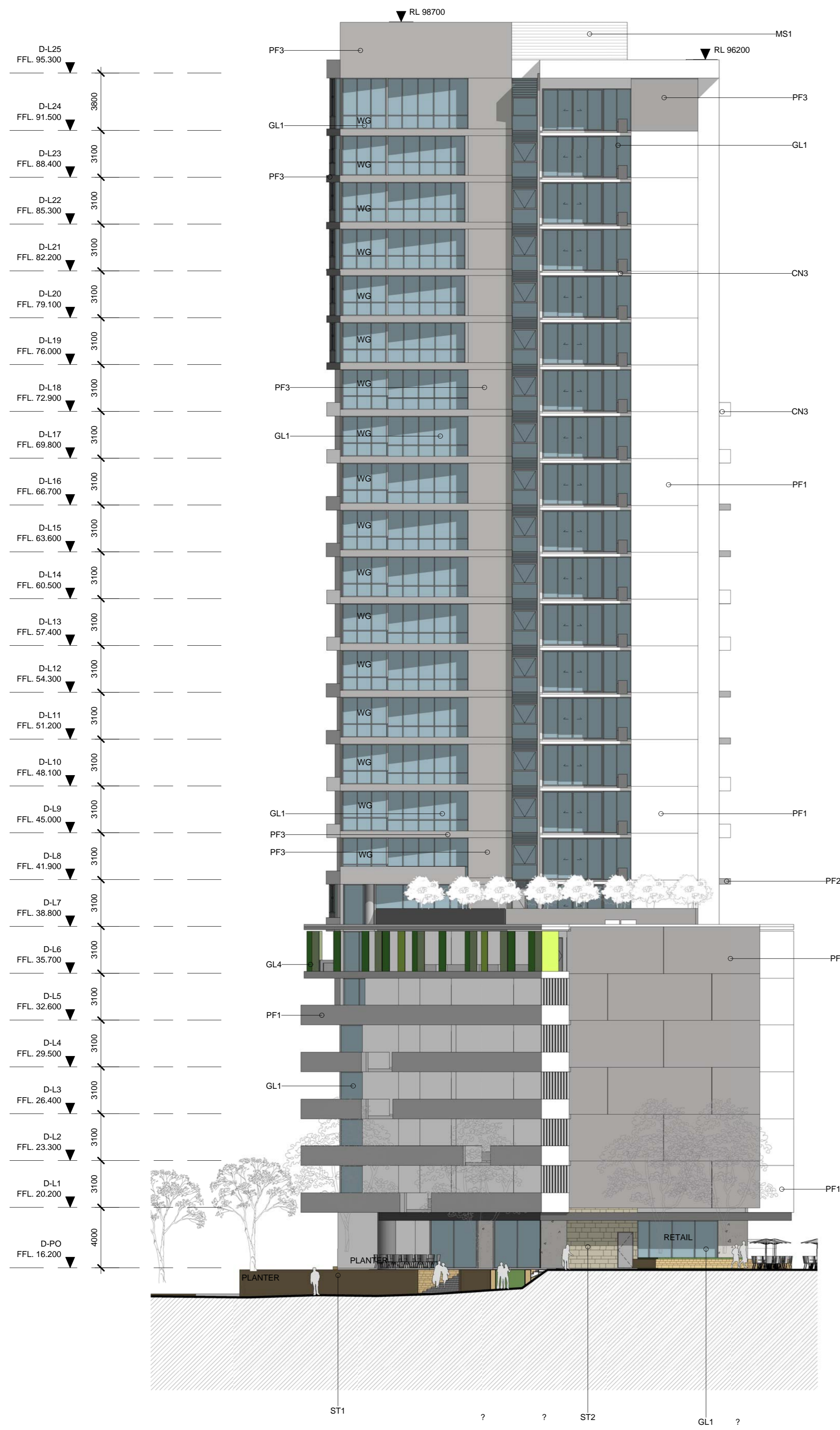
1 ELEVATION A-0201 BLDG D - NORTH 1 : 200
