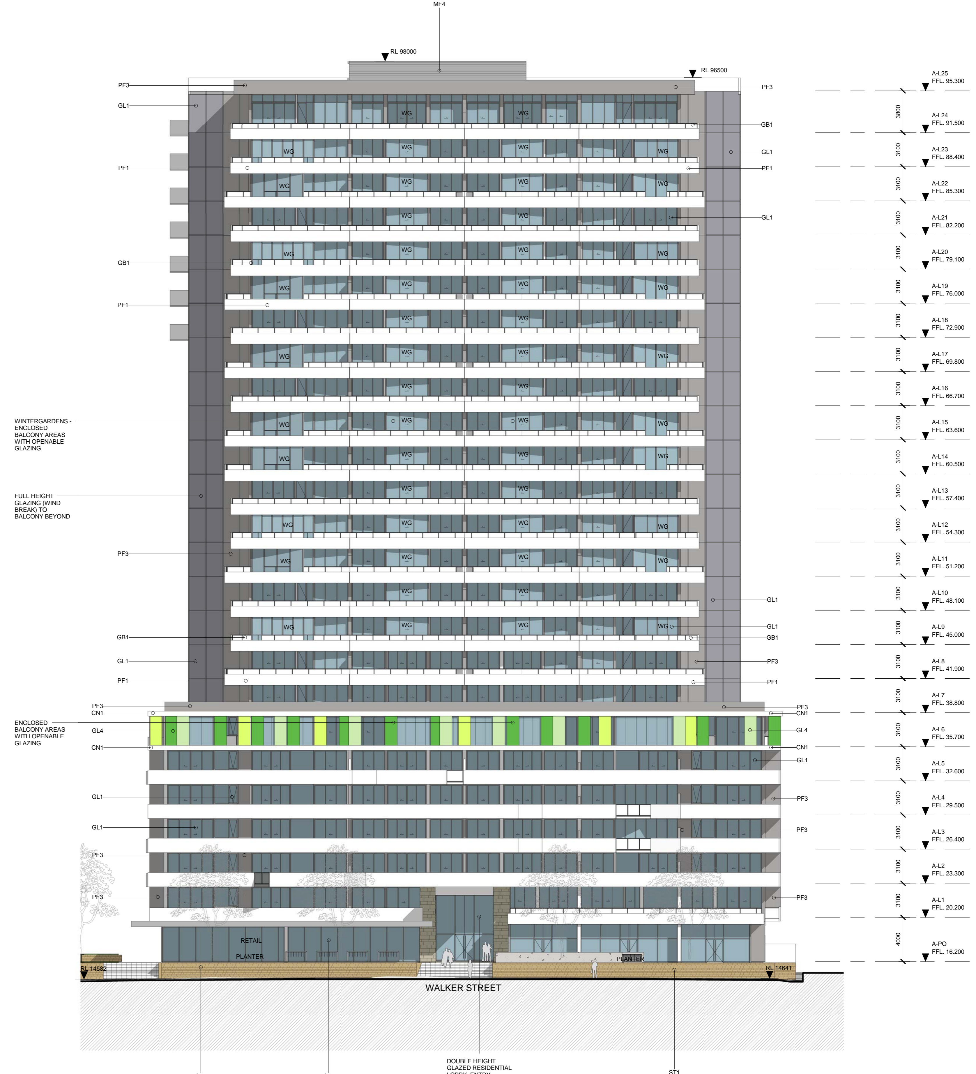
3 ELEVATION BLDG A - EAST 1:200
