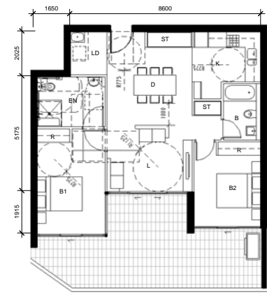
4 DETAIL PLAN BLDG A - Apartment Type 7-A Post Adaption Layout 1:100
