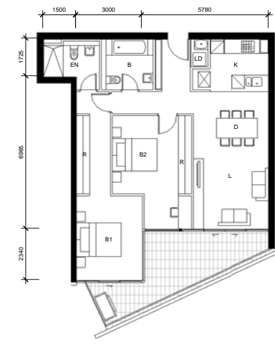
11 DETAIL PLAN BLDG D - Apartment Type 7-A Pre Adaption Layout 1:100 D.1.07 D.6.07 D.2.07 D.7.03 D.3.07 D.8.03 D.4.07 D.5.07
