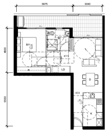
10 DETAIL PLAN BLDG D - Apartment Type 12-A Post Adaption Layout 1:100
