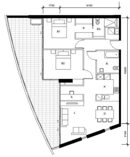
7 DETAIL PLAN BLDG C - Apartment Type 1-A Pre Adaption Layout 1:100 C.1.03 C.3.03 C.1.06 C.3.06 C.2.03 C.4.03 C.2.06 C.4.06
