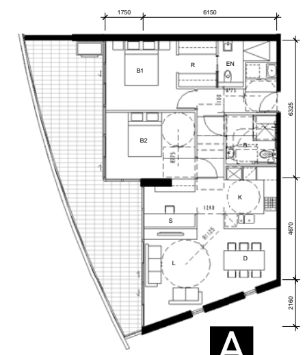
8 DETAIL PLAN BLDG C - Apartment Type 1-A Post Adaption Layout 1:100
