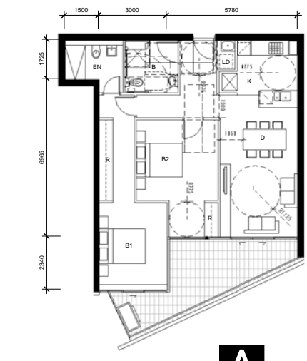
12 DETAIL PLAN BLDG D - Apartment Type 7-A Post Adaption Layout 1:100
