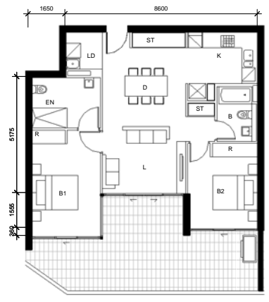
3 DETAIL PLAN BLDG A - Apartment Type 7-A Pre Adaption Layout 1:100 A.2.06 A.4.06 A.2.07 A.4.07 A.3.06 A.5.06 A.3.07 A.5.07
