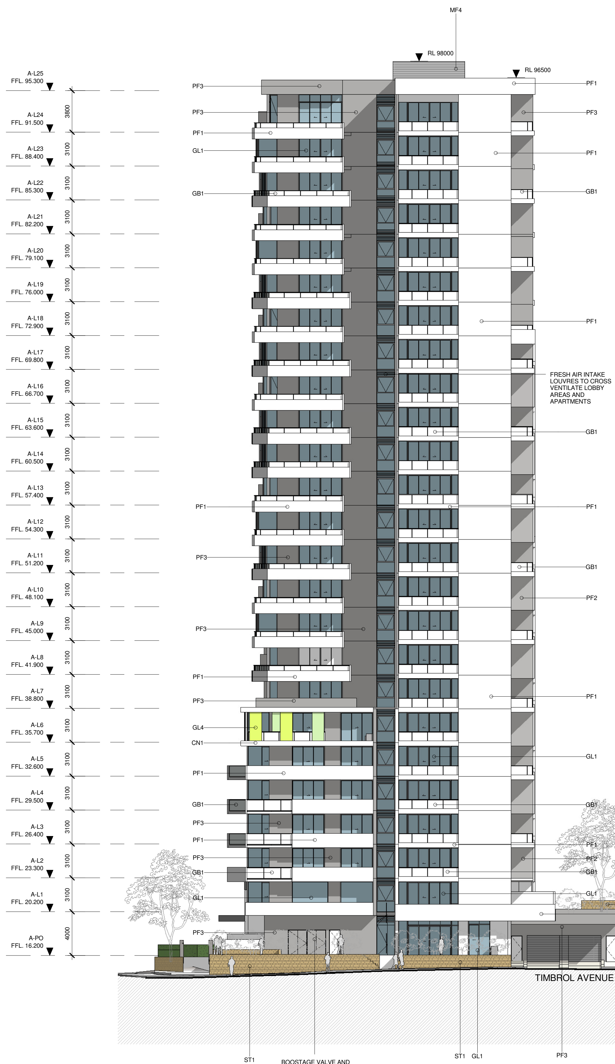
1 ELEVATION BLDG A - NORTH
