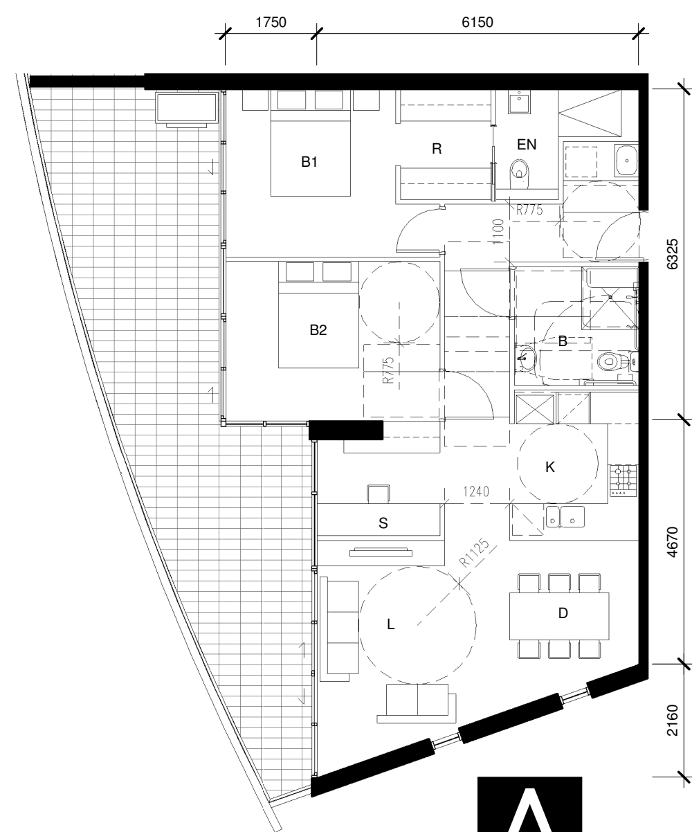
8 DETAIL PLAN BLDG C - Apartment Type 1-A Post Adaption Layout
