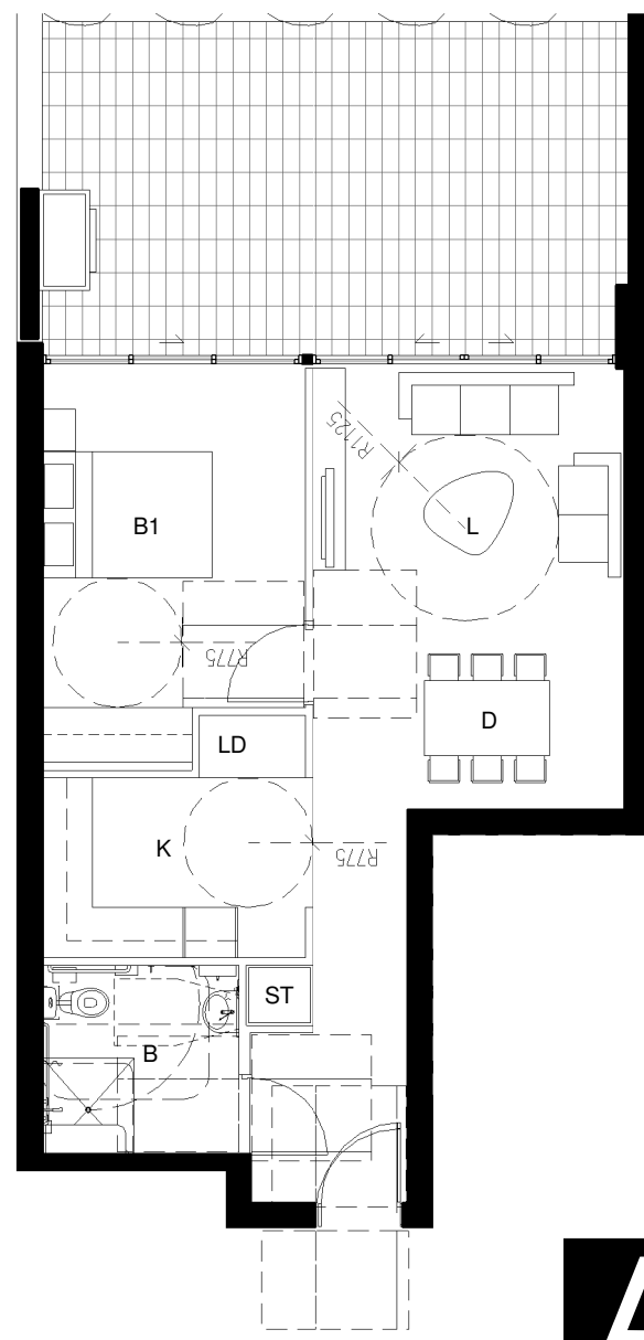
2 DETAIL PLAN BLDG A - Apartment Type 2-A Post Adaption Layout
