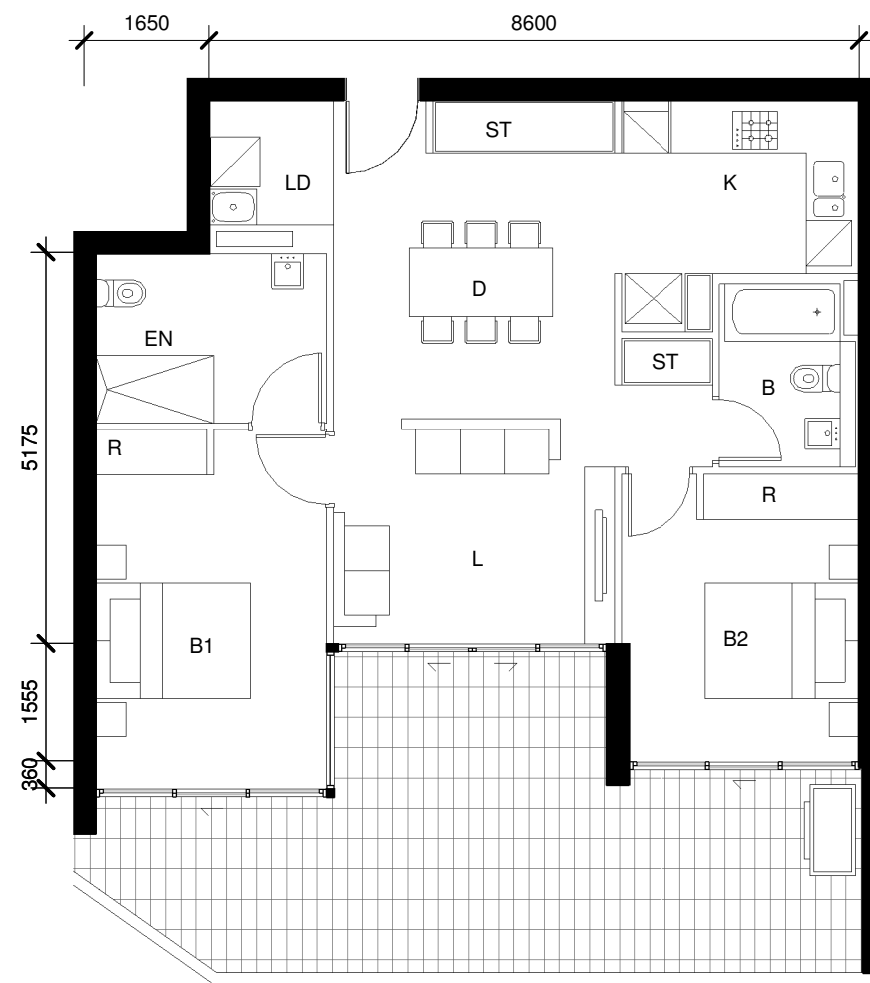
3 DETAIL PLAN BLDG A - Apartment Type 7-A Pre Adaption Layout
