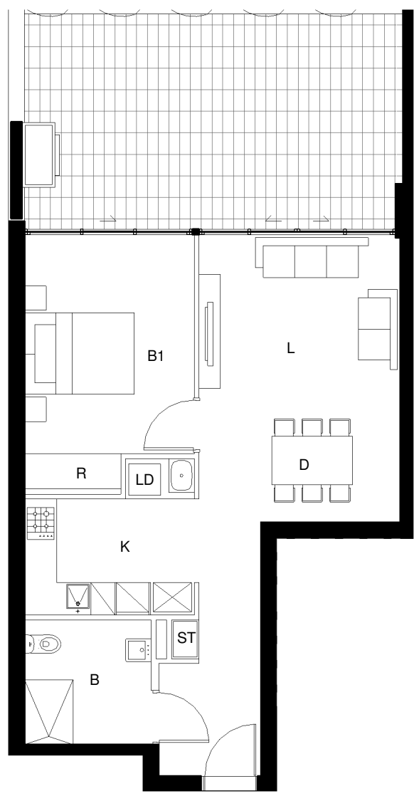
1 DETAIL PLAN BLDG A - Apartment Type 2-A Pre Adaption Layout
