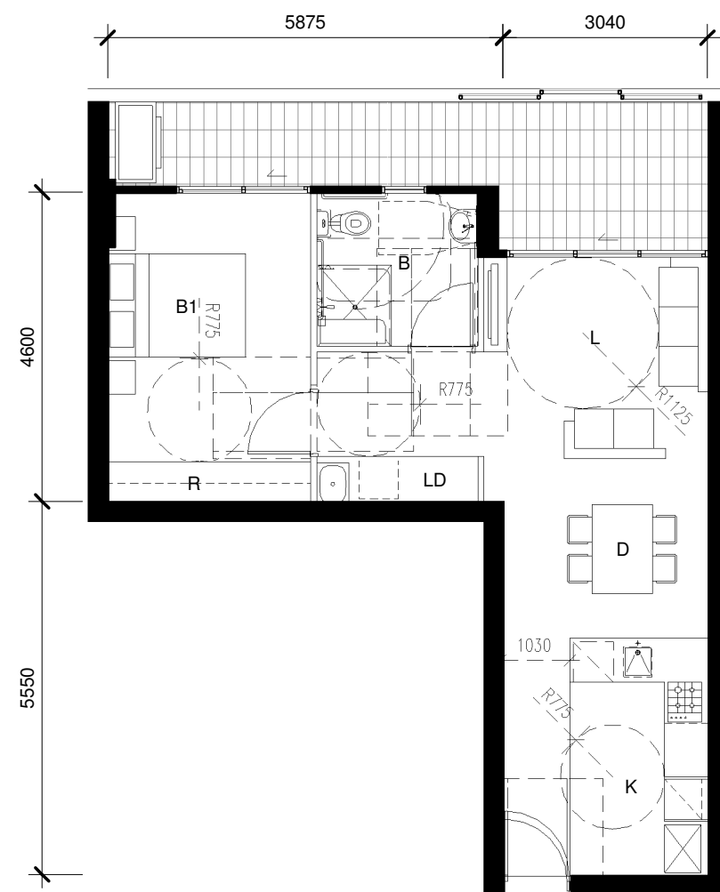
10 DETAIL PLAN BLDG D - Apartment Type 12-A Post Adaption Layout
