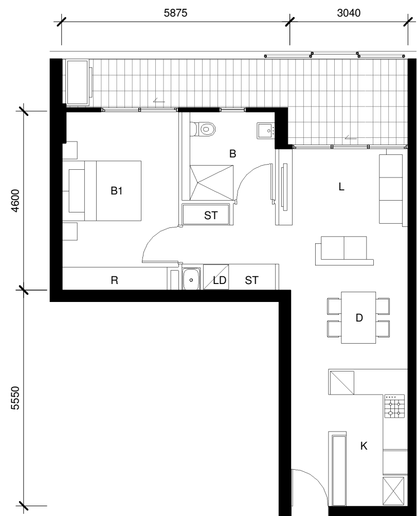
9 DETAIL PLAN BLDG D - Apartment Type 12-A Pre Adaption Layout
