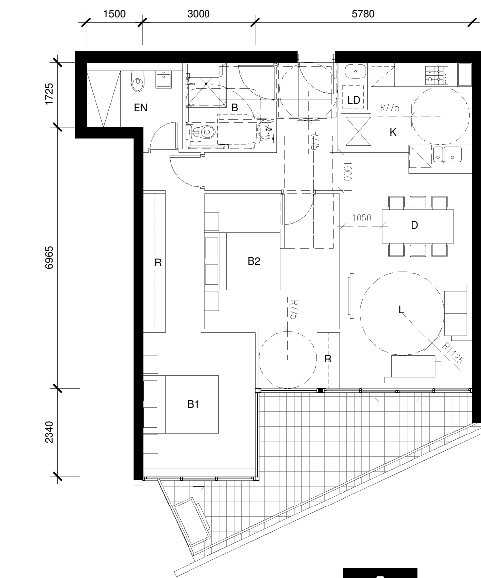
12 DETAIL PLAN BLDG D - Apartment Type 7-A Post Adaption Layout
