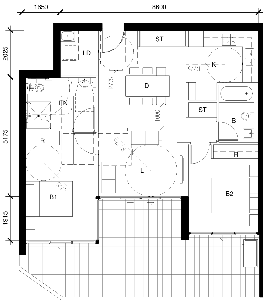
4 DETAIL PLAN BLDG A - Apartment Type 7-A Post Adaption Layout
