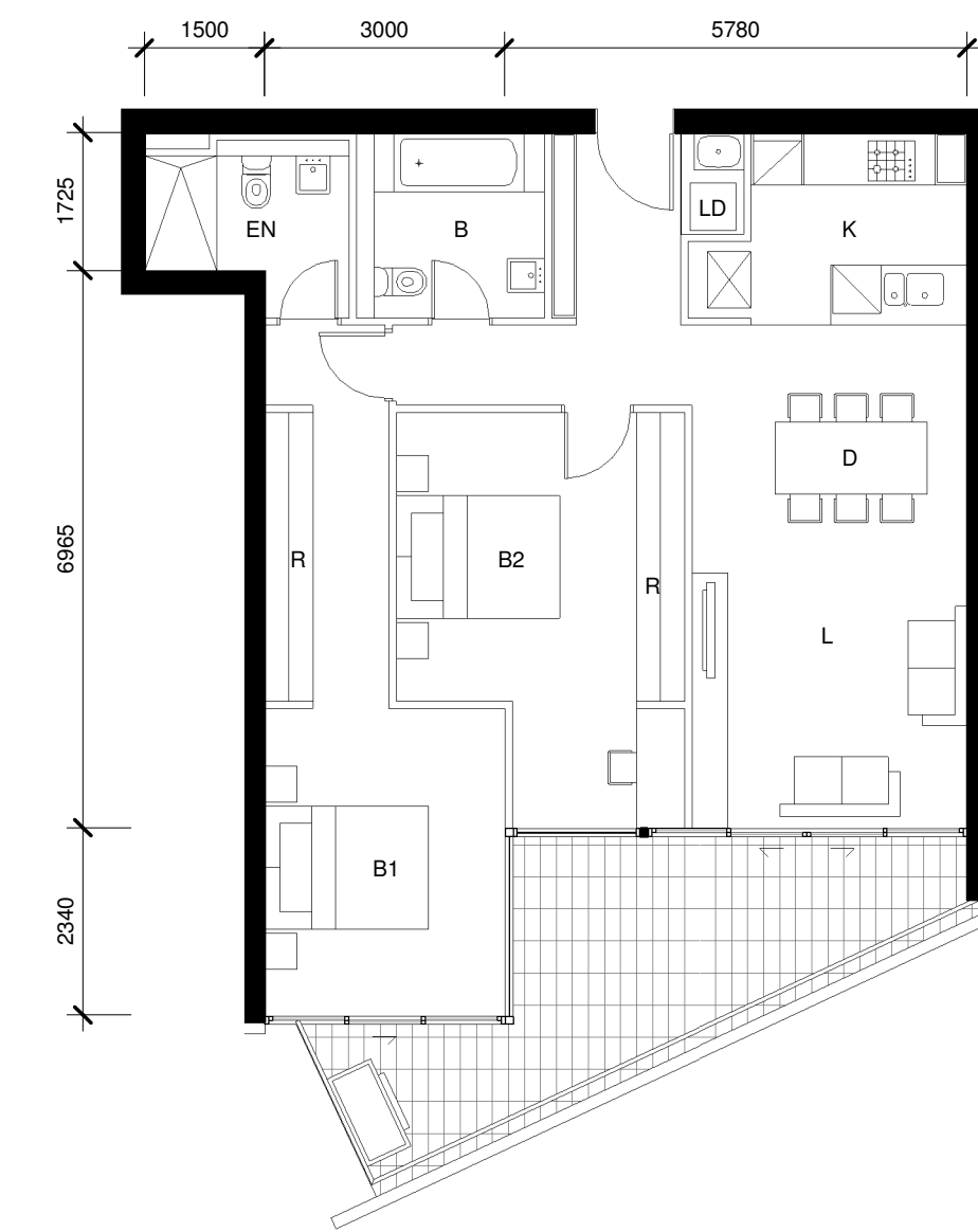
11 DETAIL PLAN BLDG D - Apartment Type 7-A Pre Adaption Layout
