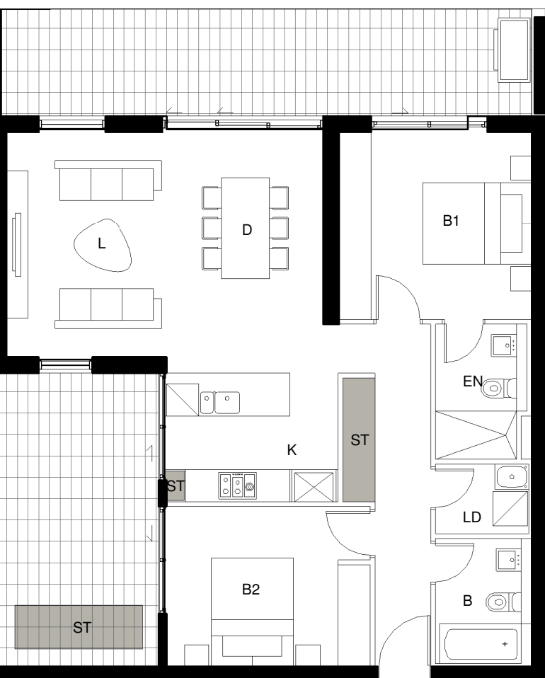
5 DETAIL PLAN BLDG A - Apartment Type 1 2 BED - 80sqm Storage - 4cbm (2cbm internal + 2cbm balcony)
