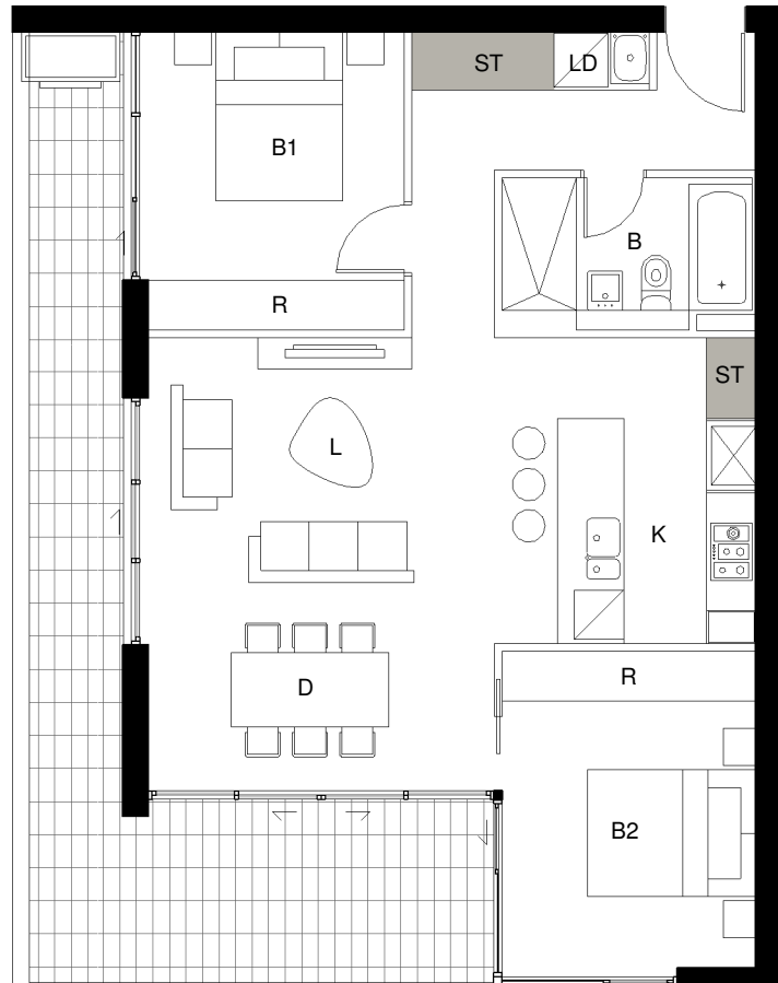
7 DETAIL PLAN BLDG A - Apartment Type 5 2 BED - 74sqm Storage - 4.8cbm
