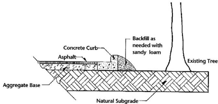
Figure 1 – Suggested method of pavement construction within TPZ's of Trees T7-T13.
