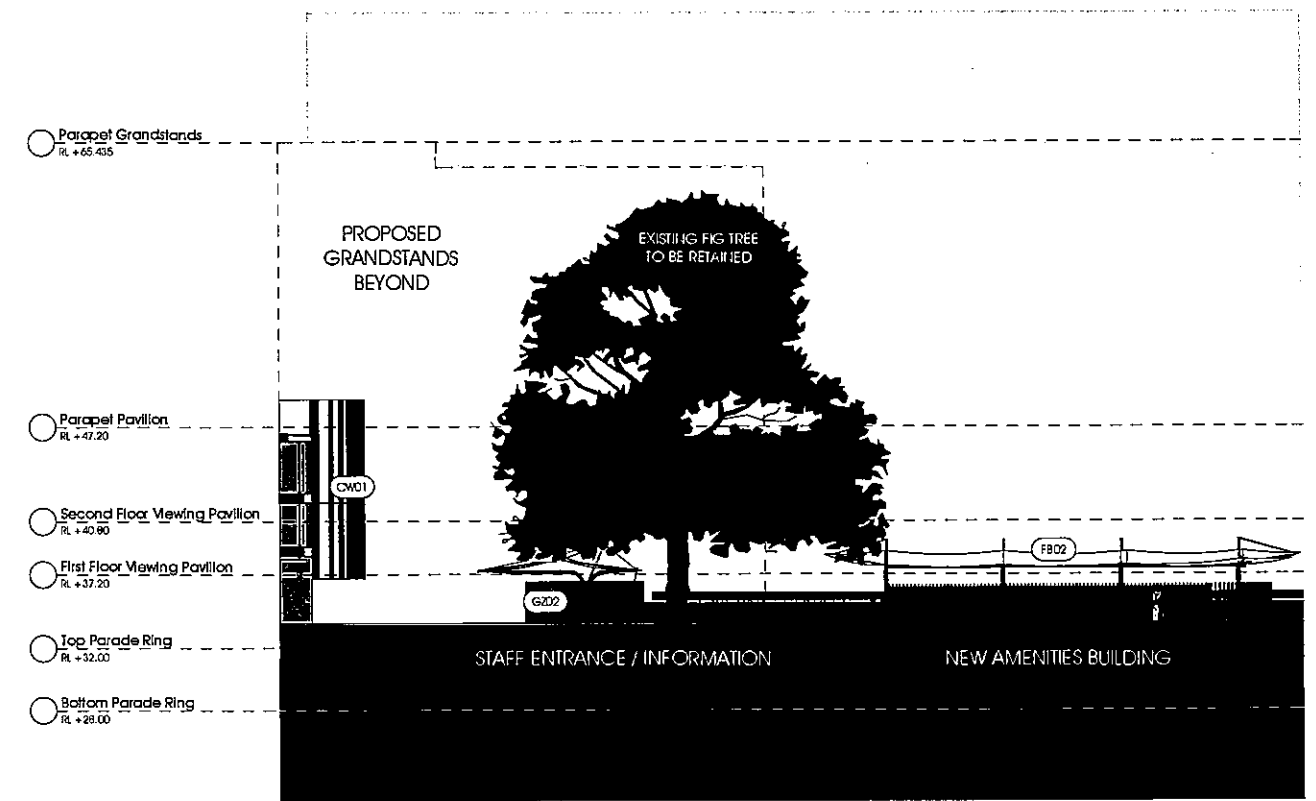
03 PARADE RING SECTION E-E
