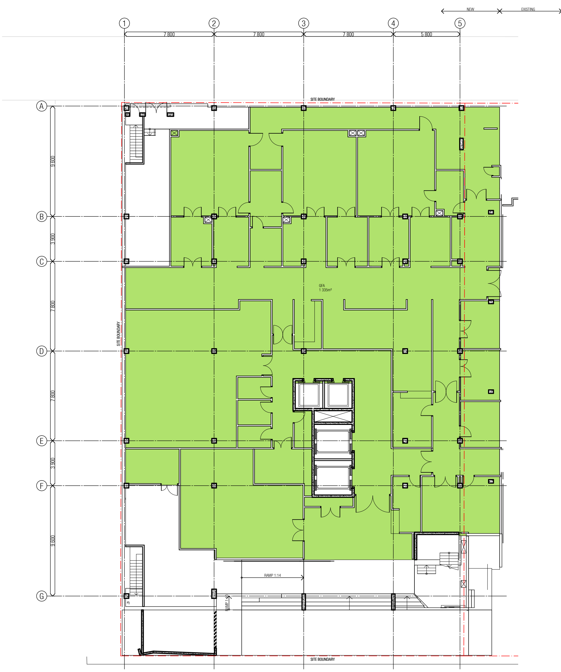
01 PLAN - GFA LEVEL 01 SCALE 1:200
