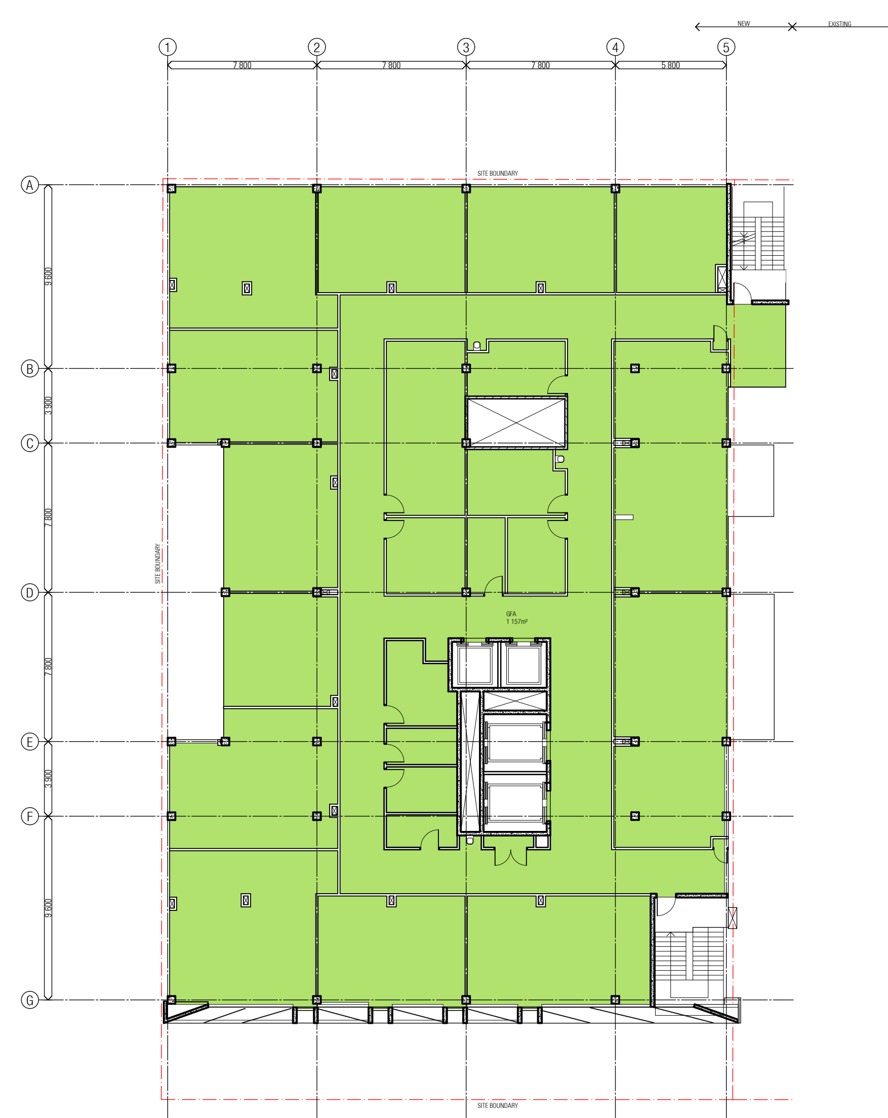
04 PLAN - GFA LEVEL 04 SCALE 1:200
