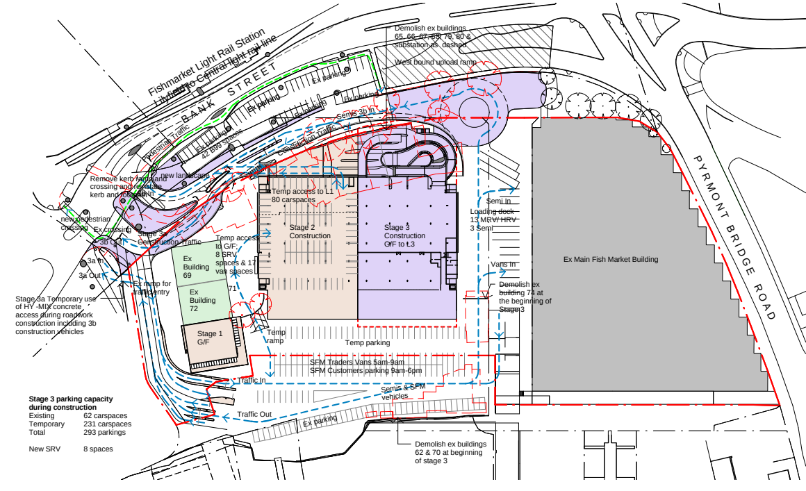
3 Site Plan Stage 3 1 : 1000
