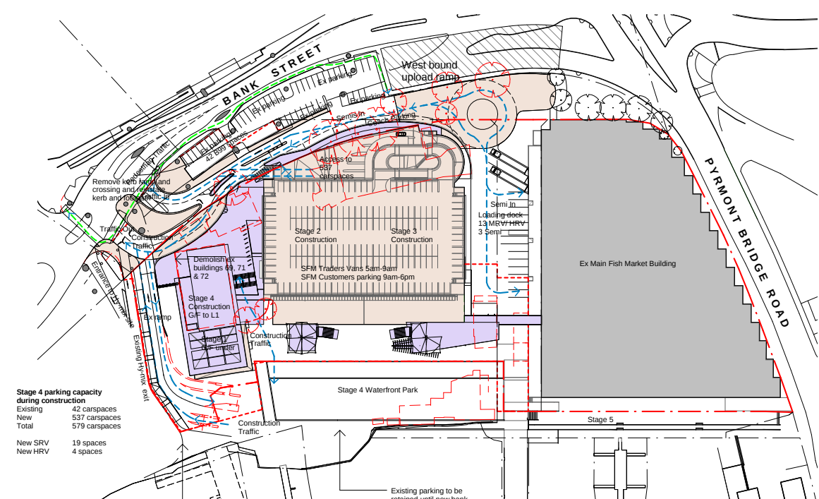
4 Site Plan Stage 4 1 : 1000
