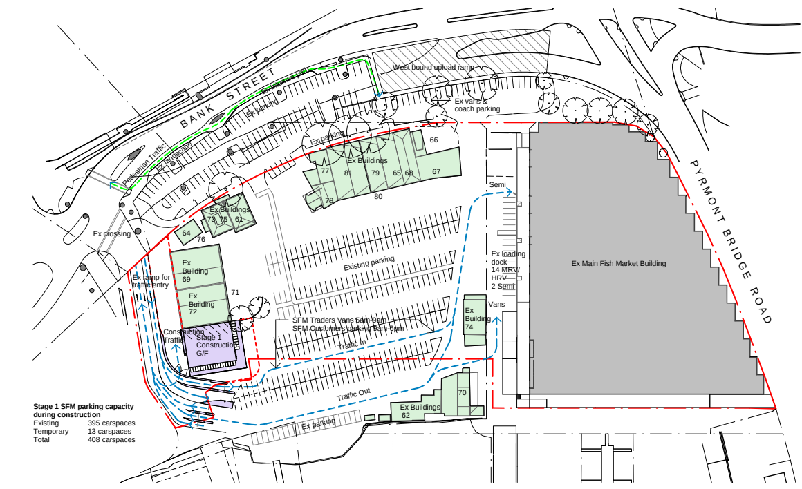
1 Site Plan Stage 1 1 : 1000
