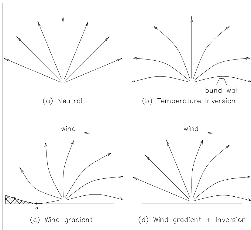
Figure A1 Sound refraction under temperature and wind gradients.
