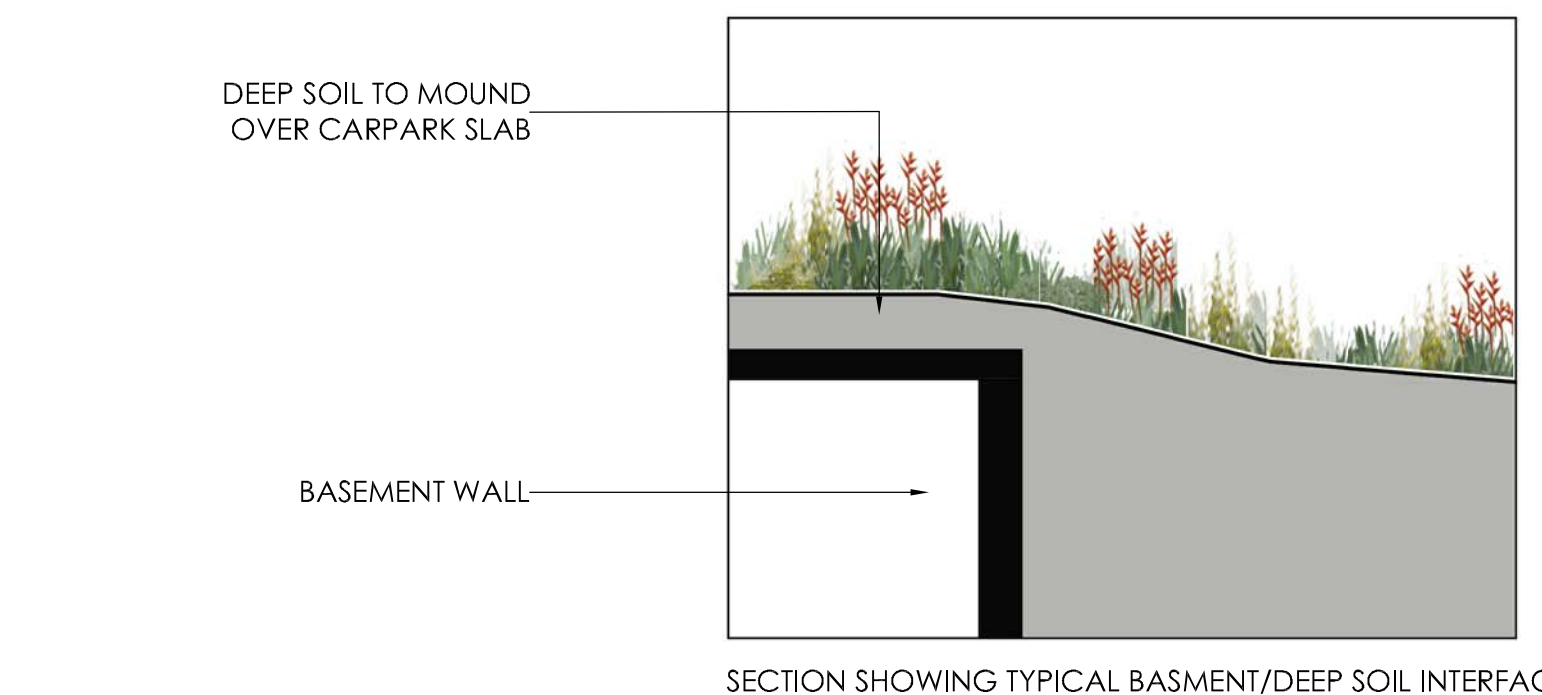
SECTION SHOWING TYPICAL BASMENT/DEEP SOIL INTERFACE
