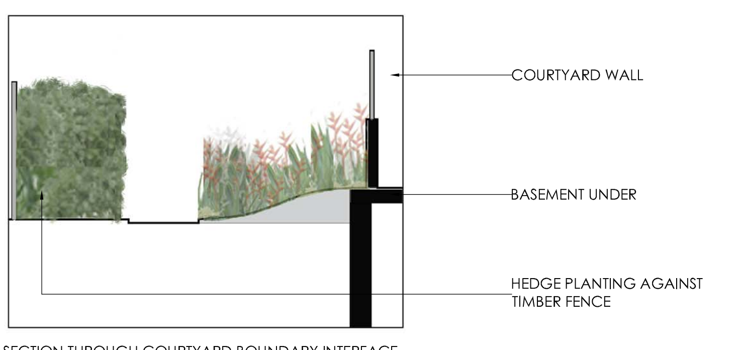
SECTION THROUGH COURTYARD BOUNDARY INTERFACE
