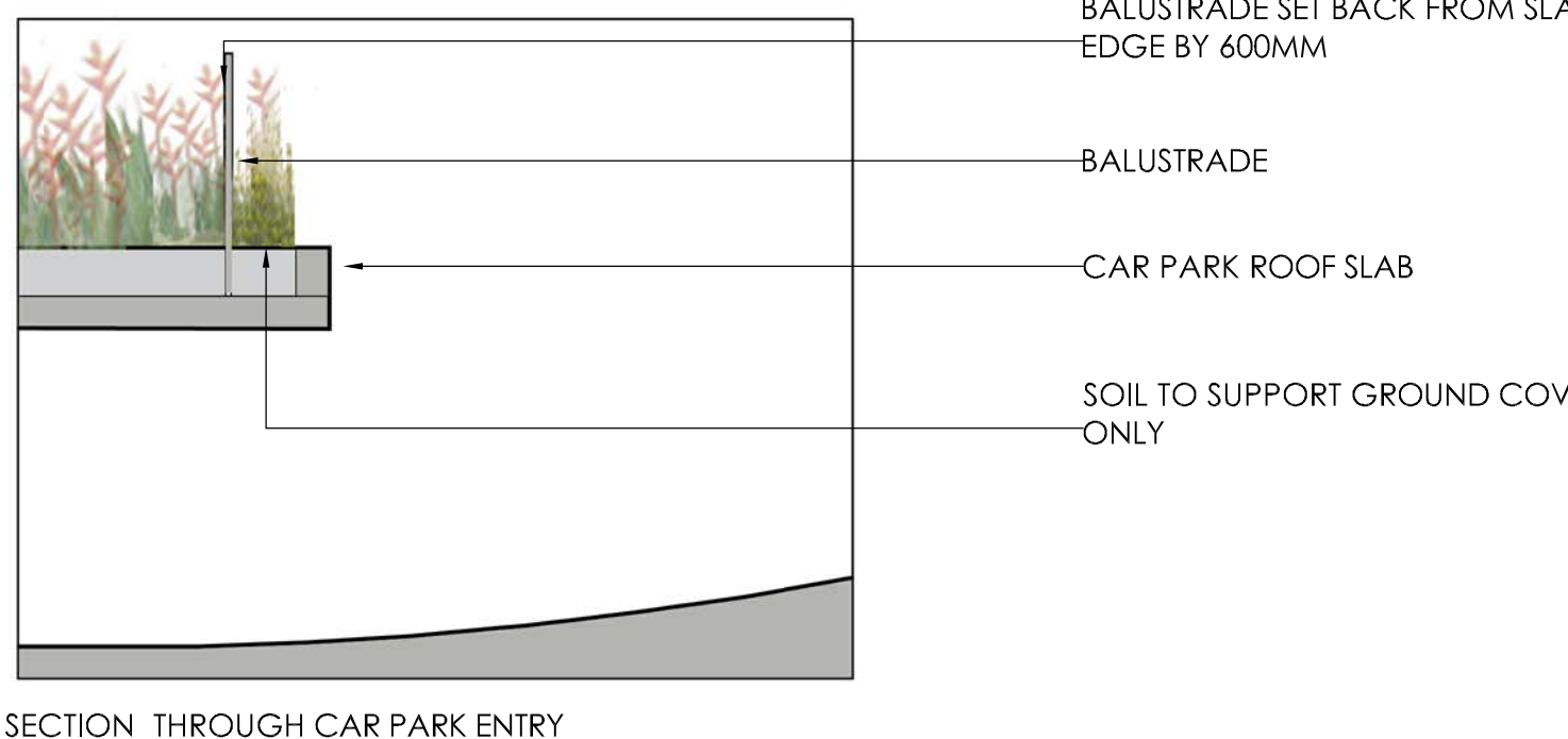
SECTION THROUGH CAR PARK ENTRY
