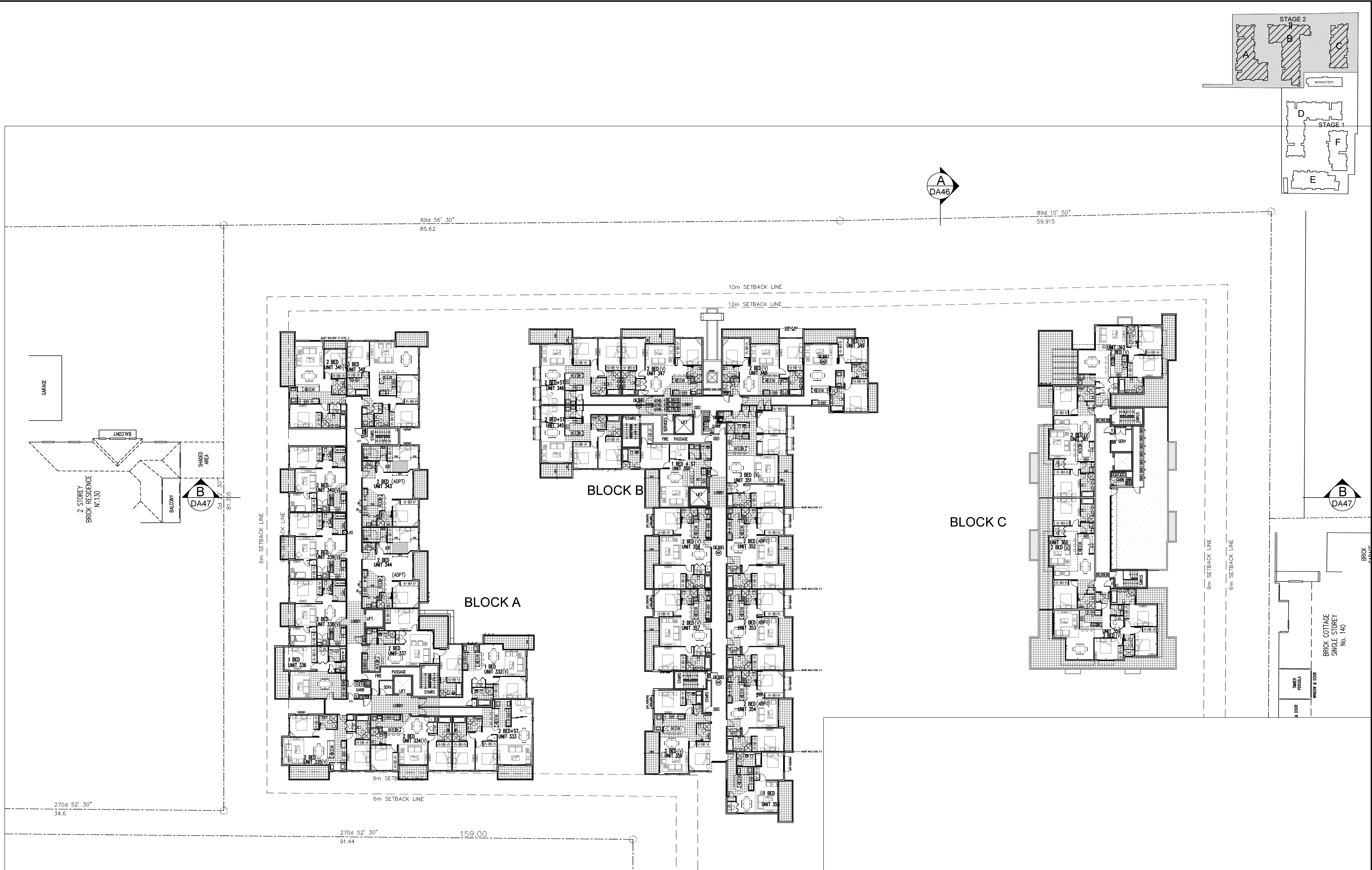
STAGE-2 LEVEL 3 PLAN SCALE 1:200
