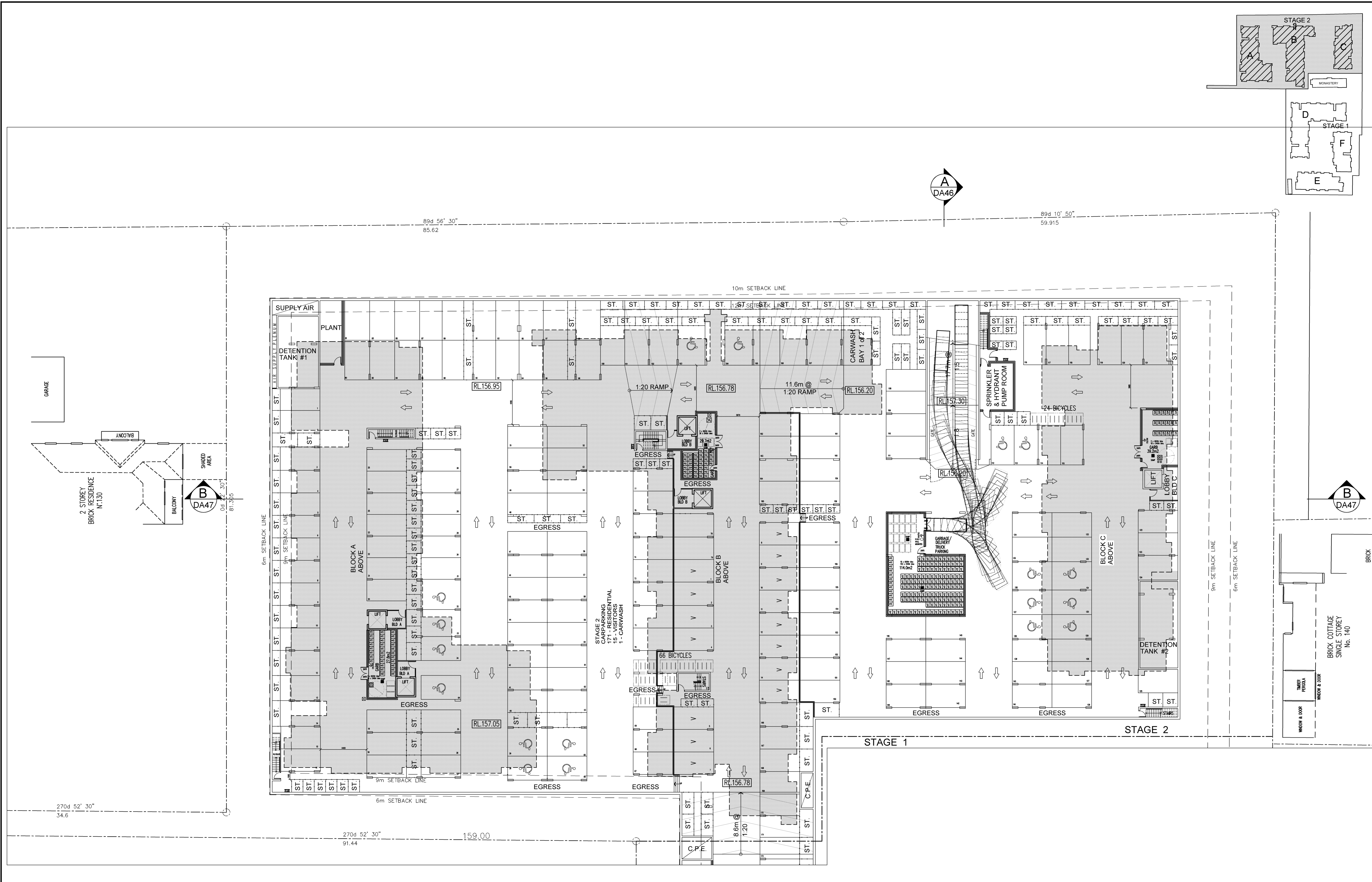
CARPARK STAGE-2 SCALE 1:200
