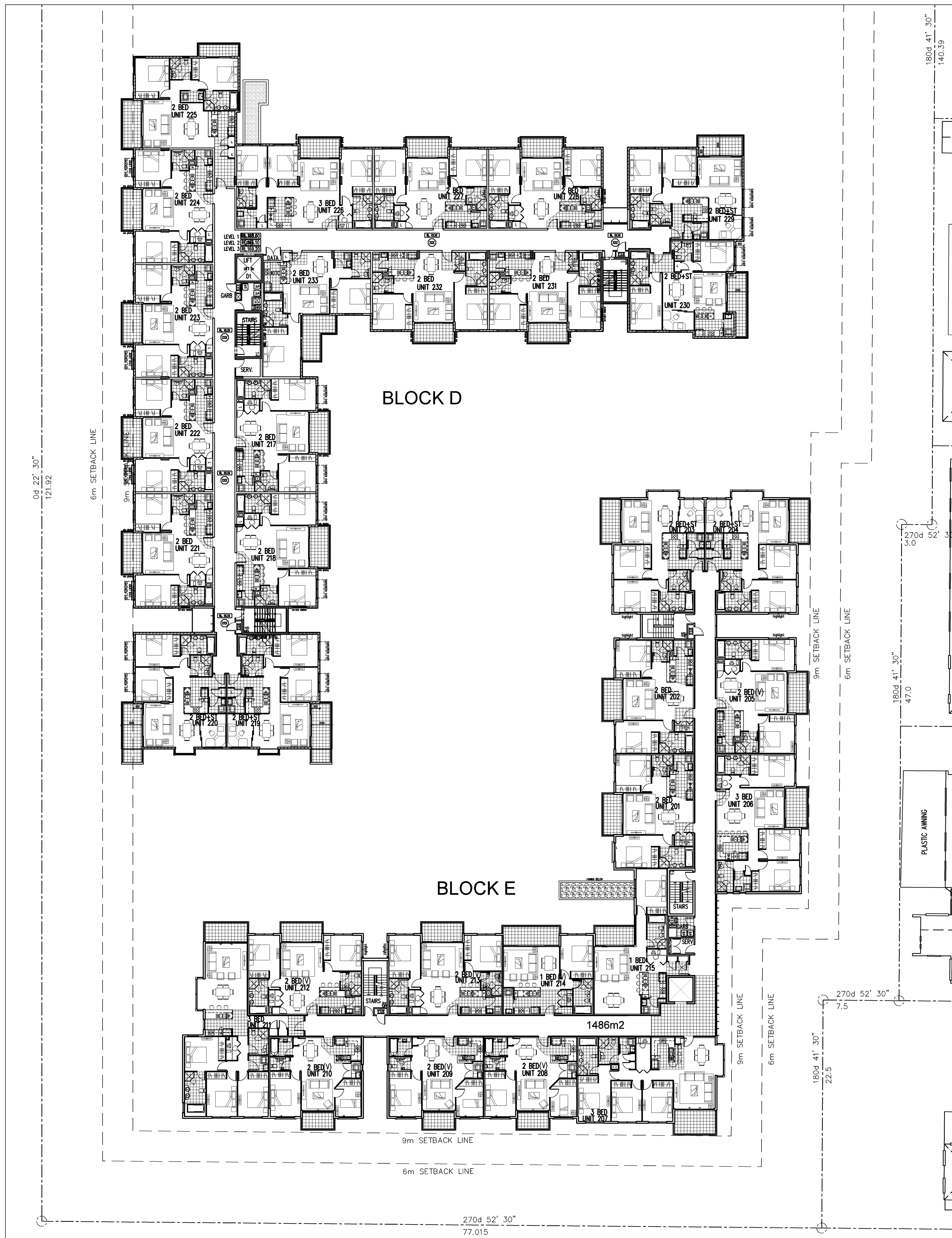
STAGE-1 LEVEL 2 PLAN
