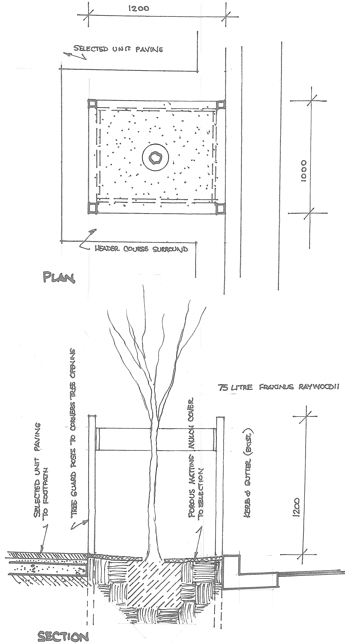
STREET TREE DETAILS 1:20
