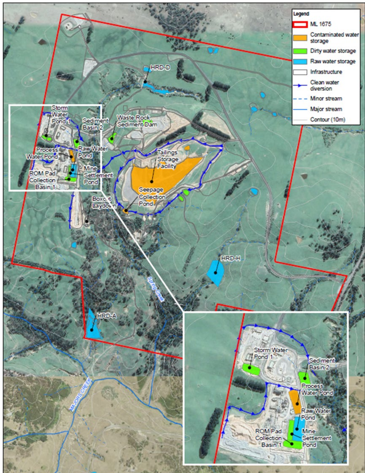
Figure 2: Mine Site Water Storages
