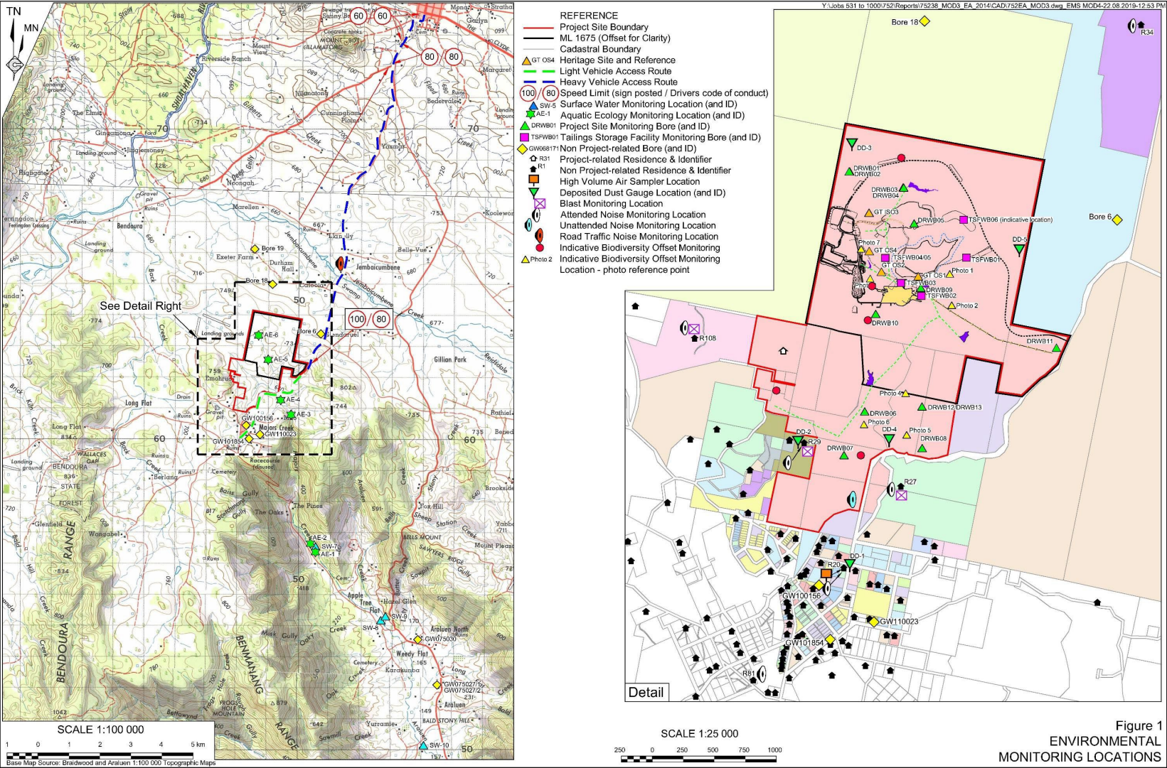
Figure 1: Environmental Monitoring Locations
