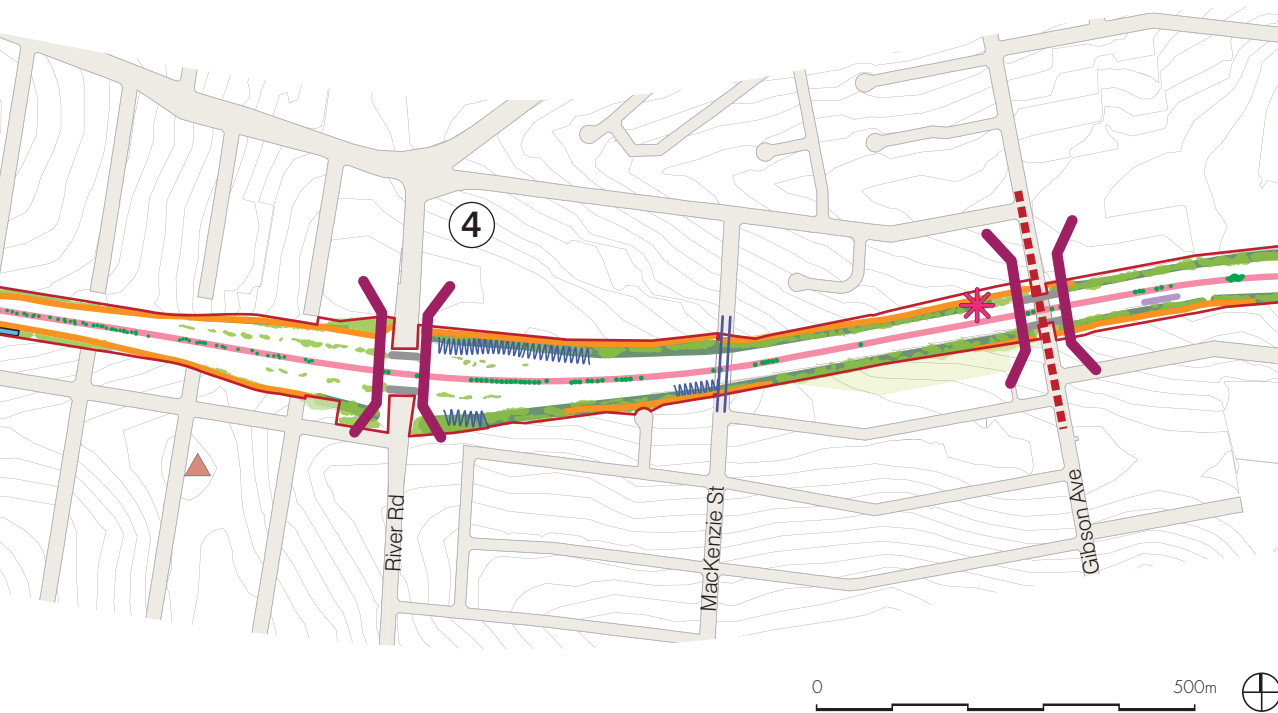
Illustration 32: Precinct 4: Existing situation overlaid with proposed upgrade works. Refer to page 29 for Legend (plan supplied by HBO+EMTB)
