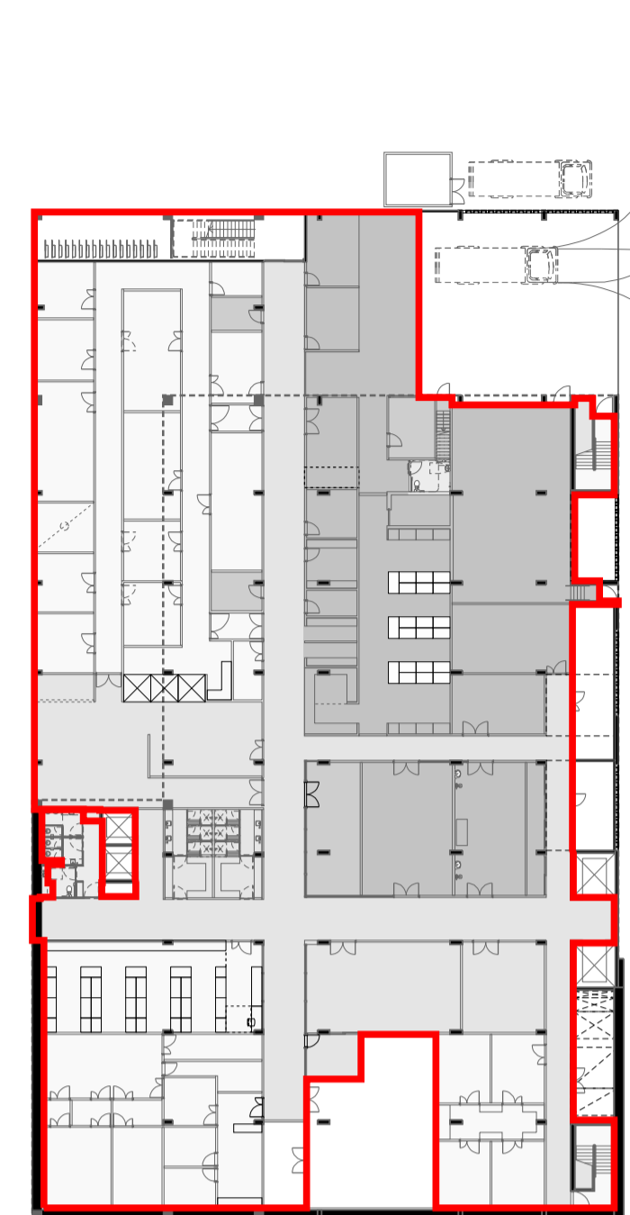
LEVEL 00 FSA APPROX. 2645 sqm
