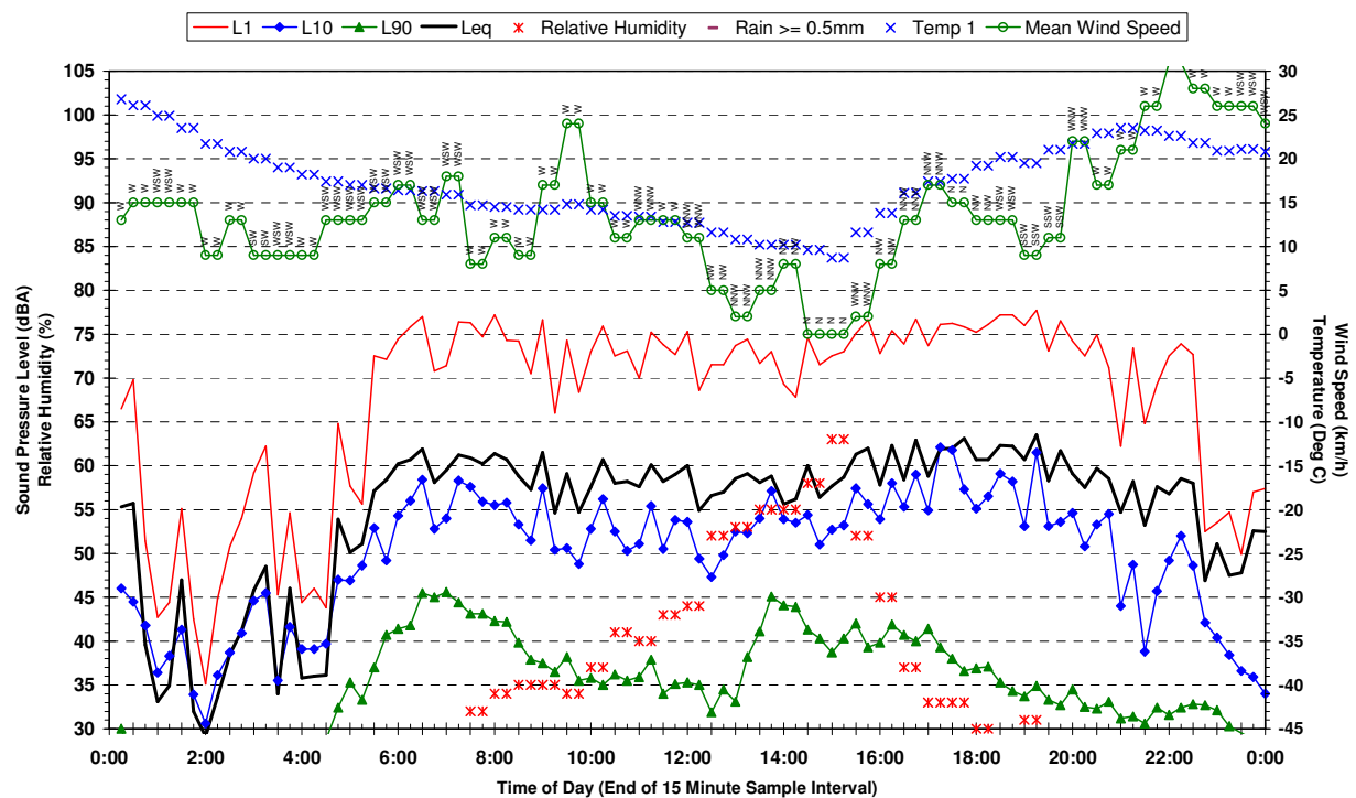
Statistical Ambient Noise Levels BG2 - 198 McCann Rd Rossmore - Friday 21 April 2006
