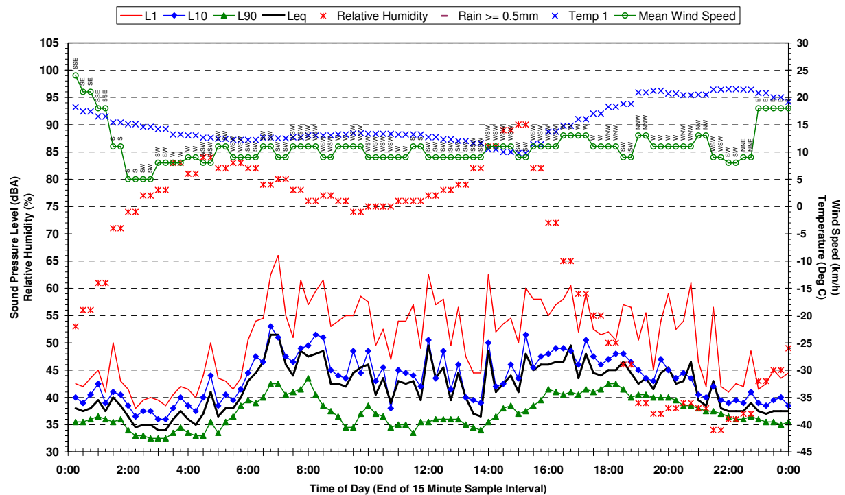
Statistical Ambient Noise Levels 25 Cassidy St Denham Court - Friday 28 April 2006
