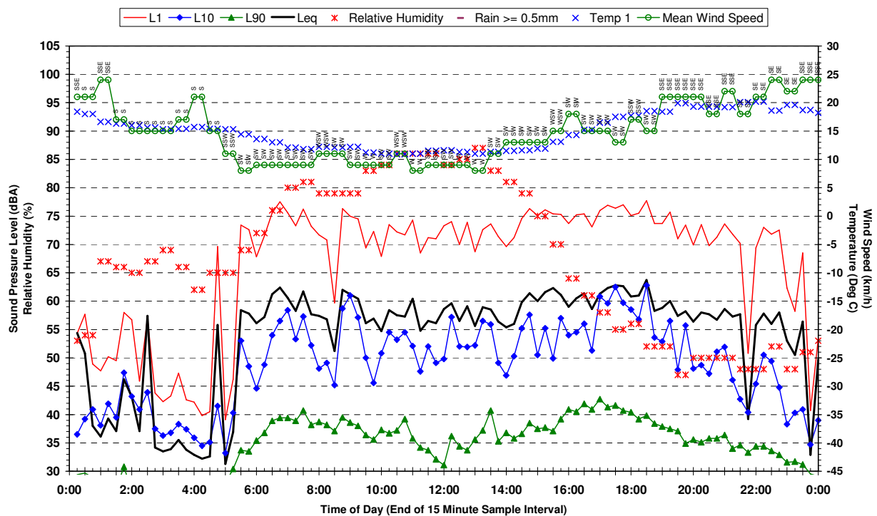
Statistical Ambient Noise Levels BG2 - 198 McCann Rd Rossmore - Thursday 27 April 2006
