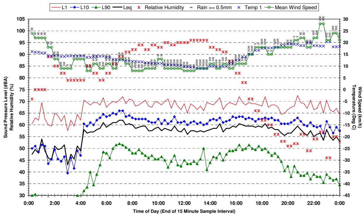
Statistical Ambient Noise Levels BG1 - 615 Bringelly Rd Rossmore - Wednesday 26 April 2006
