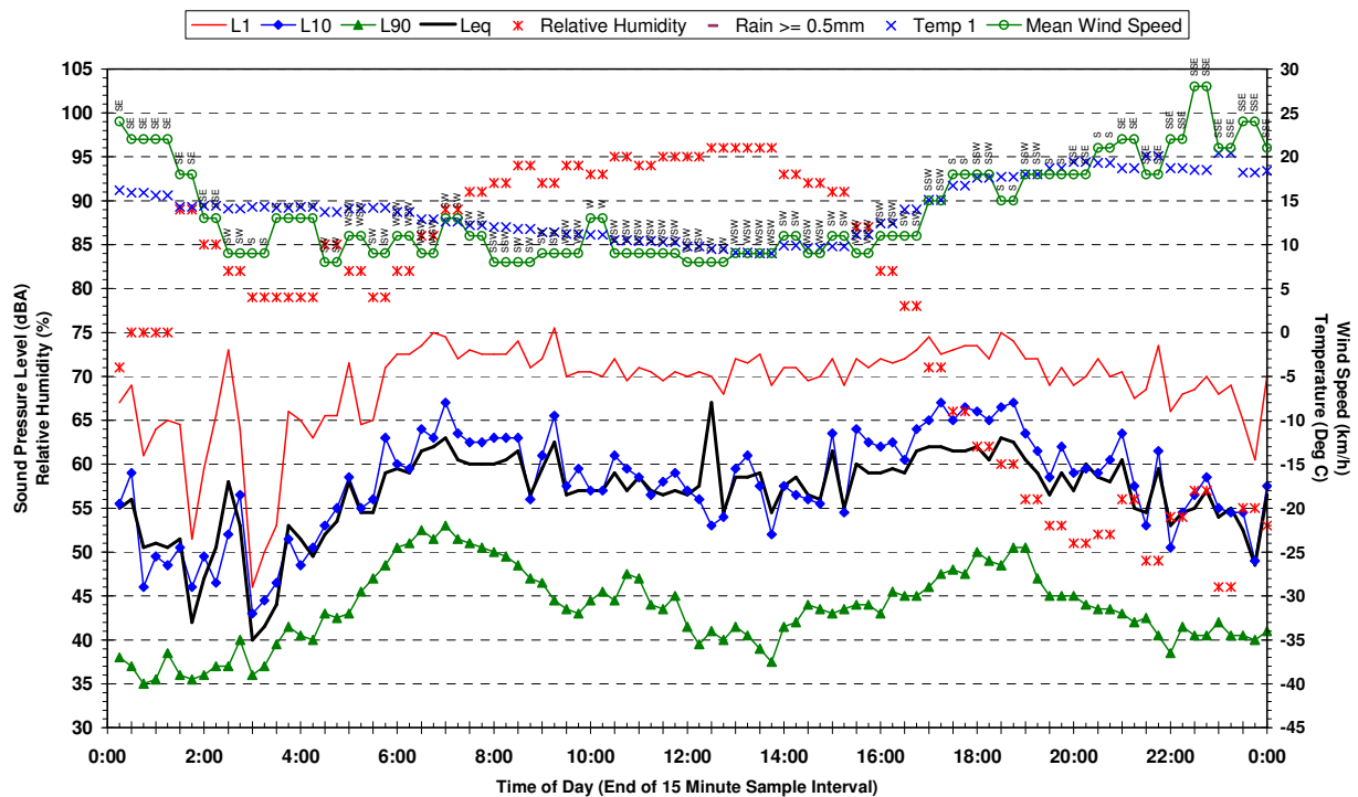
Statistical Ambient Noise Levels 18 Newtown Rd Glenfield - Wednesday 26 April 2006
