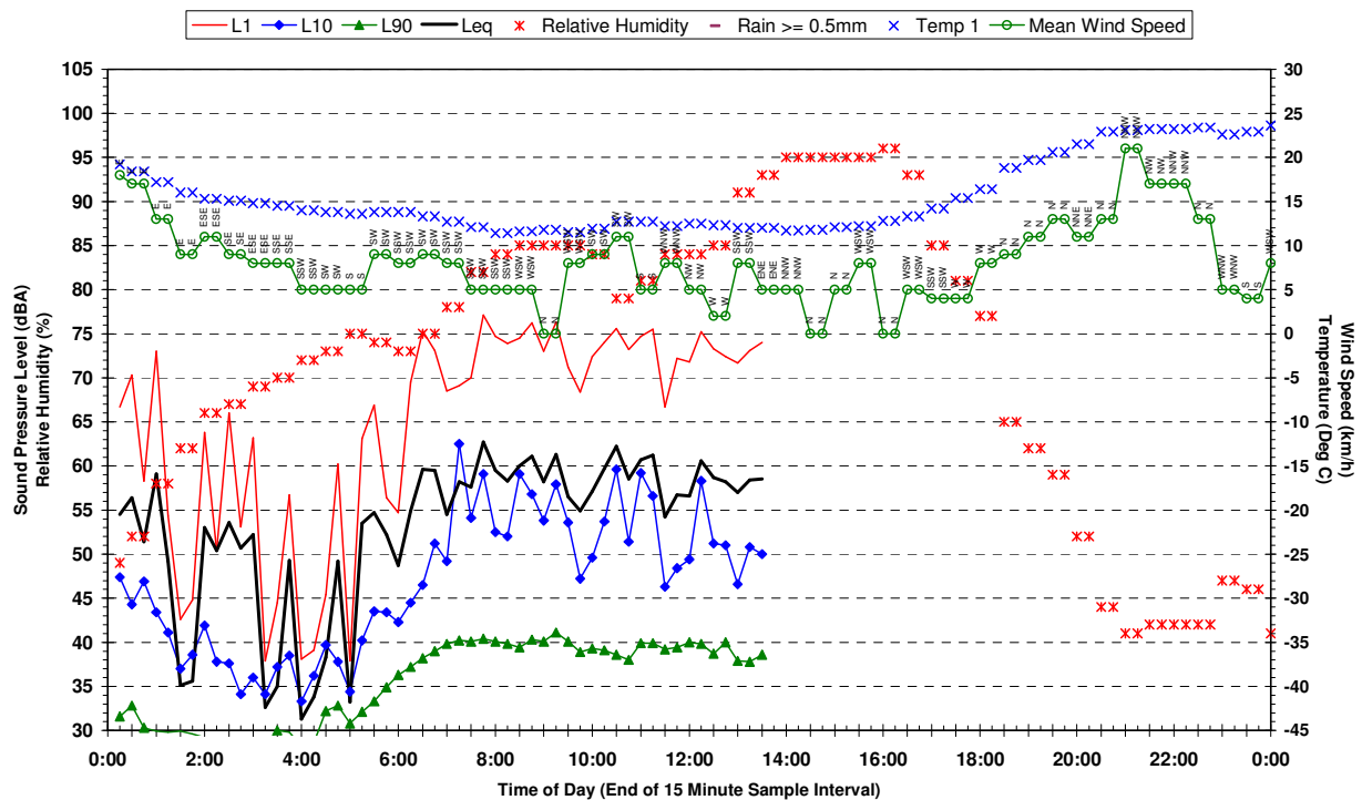
Statistical Ambient Noise Levels BG2 - 198 McCann Rd Rossmore - Saturday 29 April 2006
