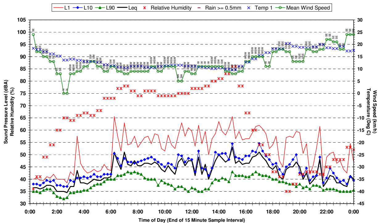
Statistical Ambient Noise Levels 25 Cassidy St Denham Court - Monday 24 April 2006
