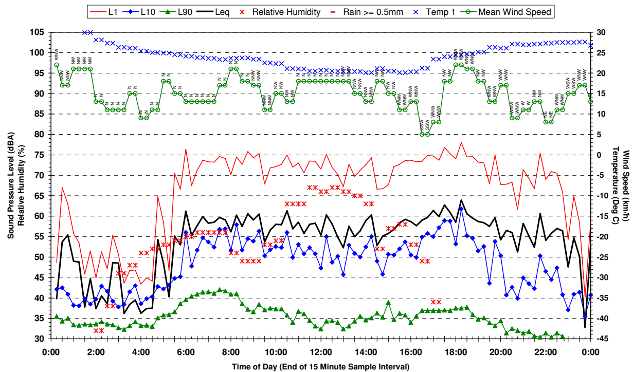
Statistical Ambient Noise Levels BG2 - 198 McCann Rd Rossmore - Thursday 20 April 2006
