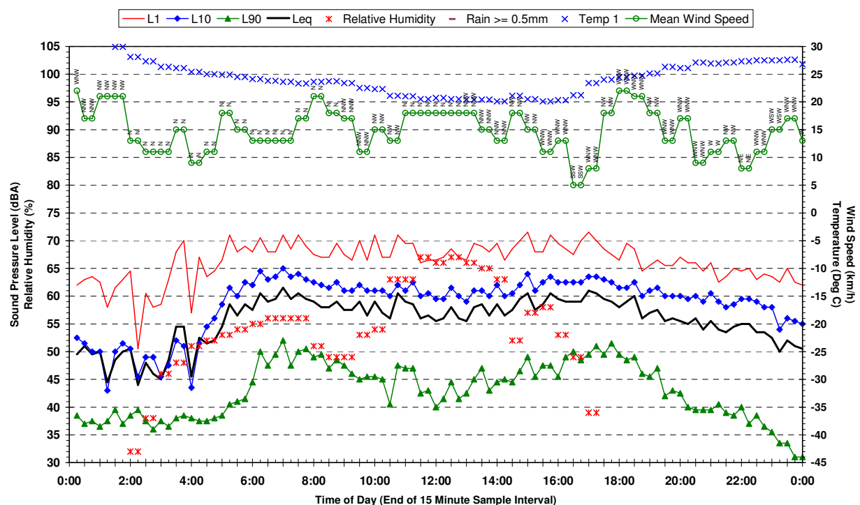
Statistical Ambient Noise Levels BG1 - 615 Bringelly Rd Rossmore - Thursday 20 April 2006
