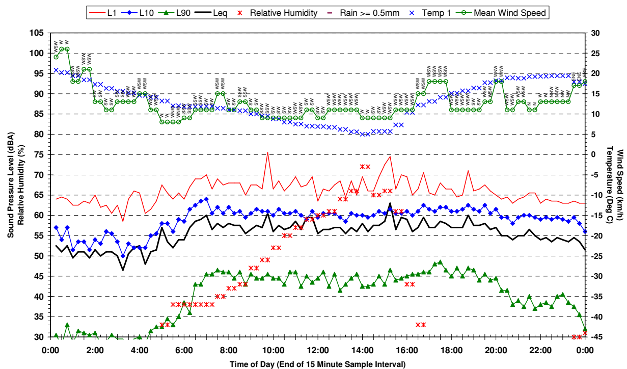
Statistical Ambient Noise Levels BG1 - 615 Bringelly Rd Rossmore - Saturday 22 April 2006
