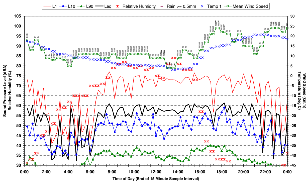
Statistical Ambient Noise Levels BG2 - 198 McCann Rd Rossmore - Sunday 23 April 2006
