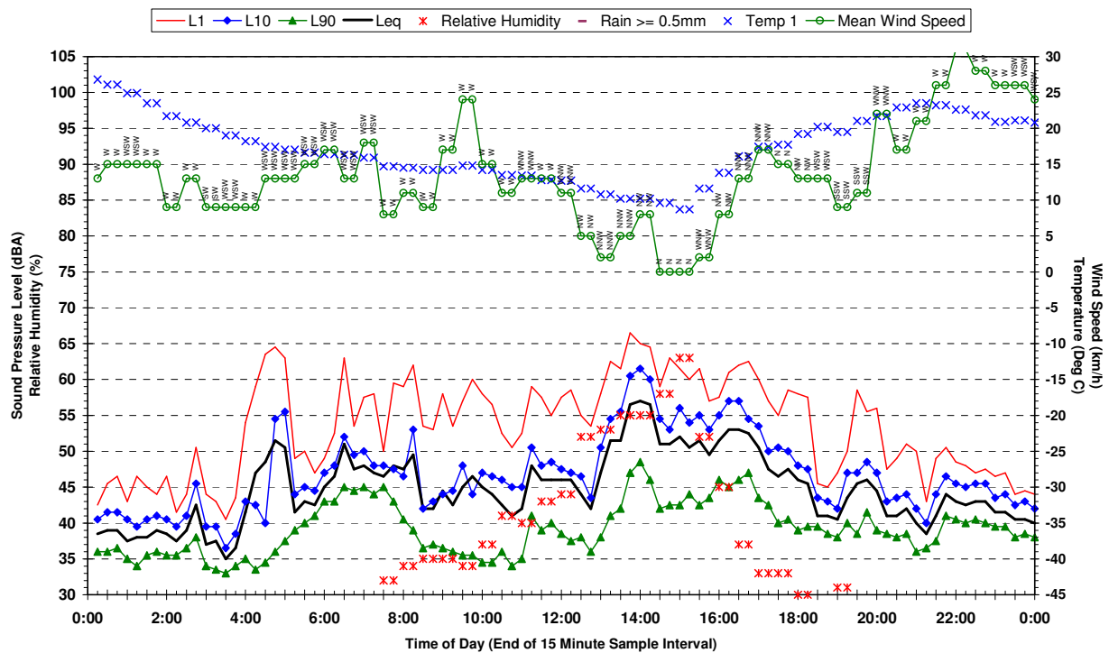
Statistical Ambient Noise Levels 25 Cassidy St Denham Court - Friday 21 April 2006
