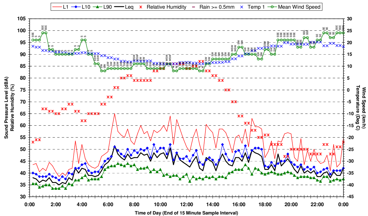
Statistical Ambient Noise Levels 25 Cassidy St Denham Court - Thursday 27 April 2006
