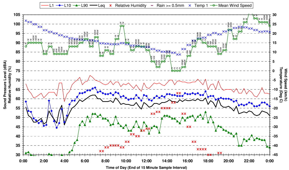
Statistical Ambient Noise Levels BG1 - 615 Bringelly Rd Rossmore - Friday 21 April 2006
