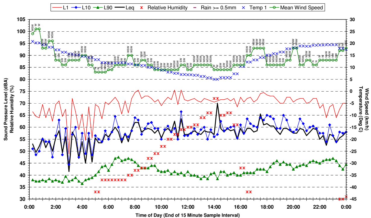
Statistical Ambient Noise Levels 18 Newtown Rd Glenfield - Saturday 22 April 2006
