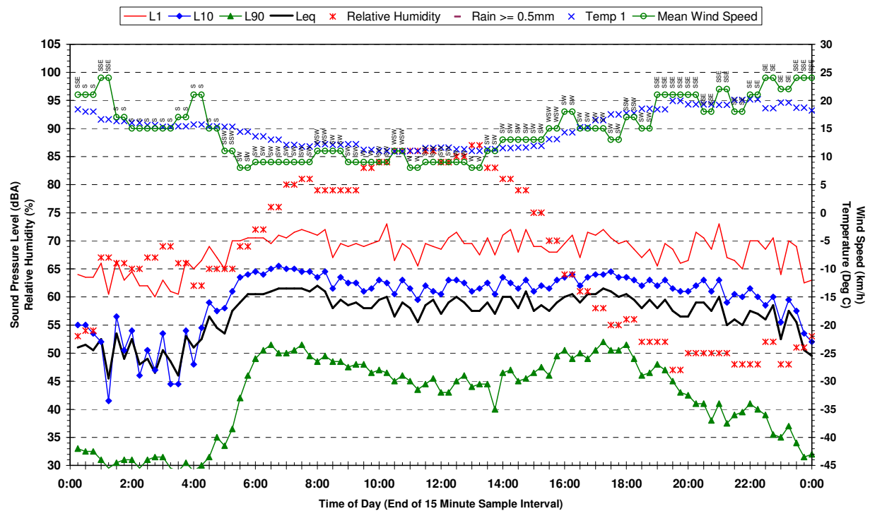
Statistical Ambient Noise Levels BG1 - 615 Bringelly Rd Rossmore - Thursday 27 April 2006
