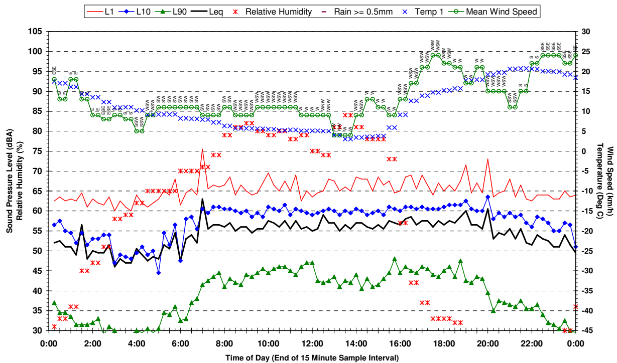
Statistical Ambient Noise Levels BG1 - 615 Bringelly Rd Rossmore - Sunday 23 April 2006
