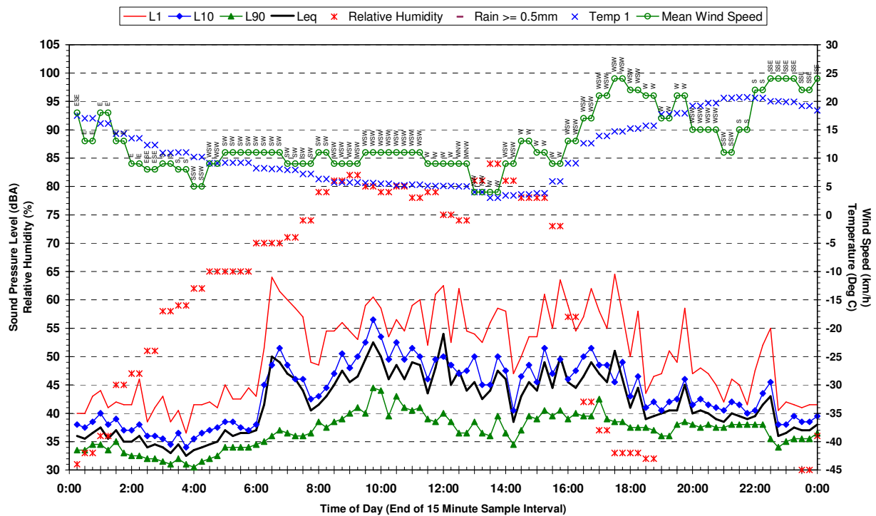
Statistical Ambient Noise Levels 25 Cassidy St Denham Court - Sunday 23 April 2006
