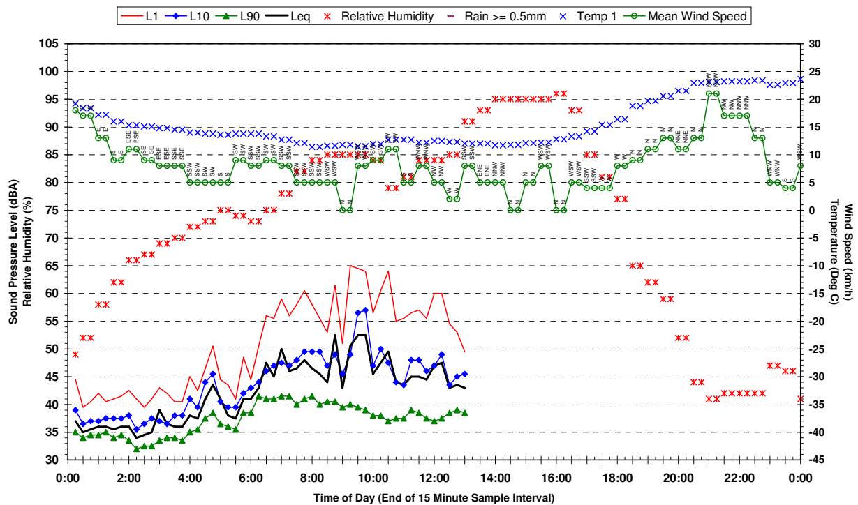
Statistical Ambient Noise Levels 25 Cassidy St Denham Court - Saturday 29 April 2006
