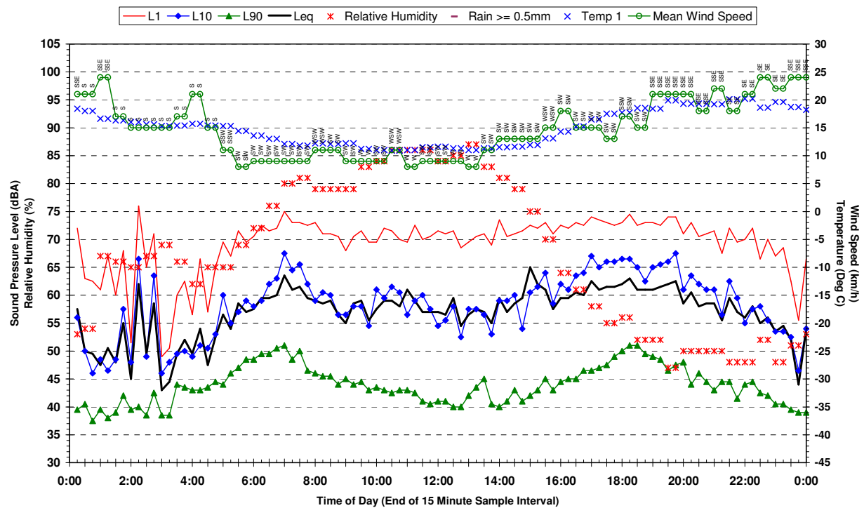
Statistical Ambient Noise Levels 18 Newtown Rd Glenfield - Thursday 27 April 2006
