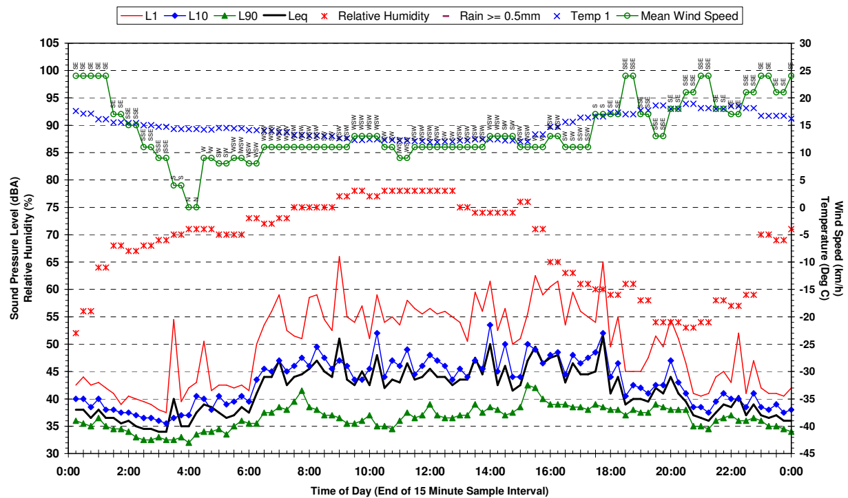
Statistical Ambient Noise Levels 25 Cassidy St Denham Court - Tuesday 25 April 2006
