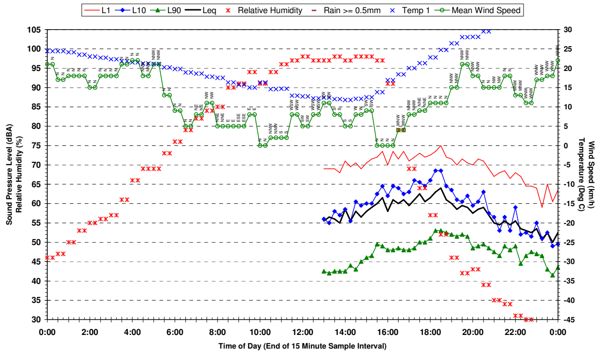
Statistical Ambient Noise Levels 18 Newtown Rd Glenfield - Wednesday 19 April 2006
