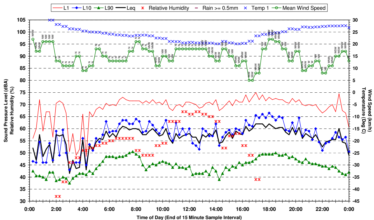
Statistical Ambient Noise Levels 18 Newtown Rd Glenfield - Thursday 20 April 2006
