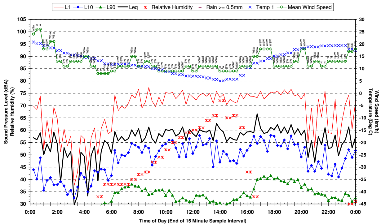
Statistical Ambient Noise Levels BG2 - 198 McCann Rd Rossmore - Saturday 22 April 2006
