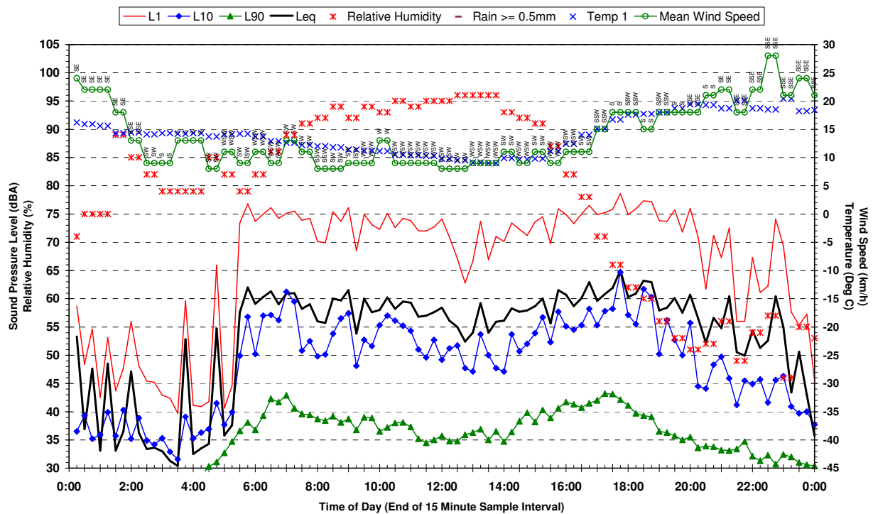
Statistical Ambient Noise Levels BG2 - 198 McCann Rd Rossmore - Wednesday 26 April 2006
