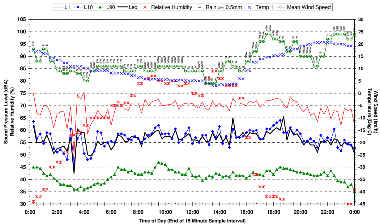
Statistical Ambient Noise Levels 18 Newtown Rd Glenfield - Sunday 23 April 2006
