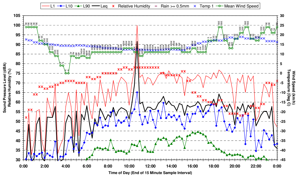
Statistical Ambient Noise Levels BG2 - 198 McCann Rd Rossmore - Tuesday 25 April 2006
