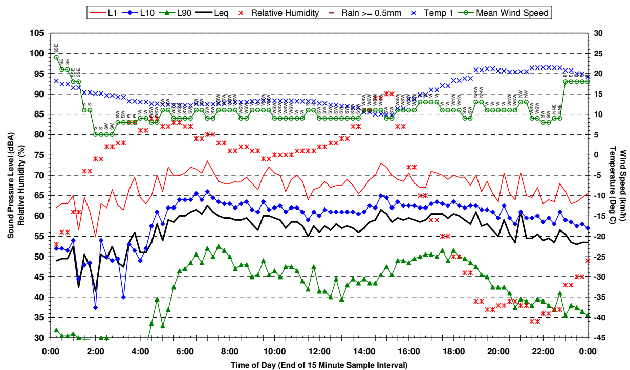
Statistical Ambient Noise Levels BG1 - 615 Bringelly Rd Rossmore - Friday 28 April 2006
