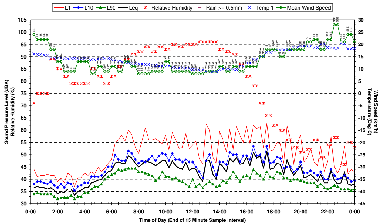
Statistical Ambient Noise Levels 25 Cassidy St Denham Court - Wednesday 26 April 2006
