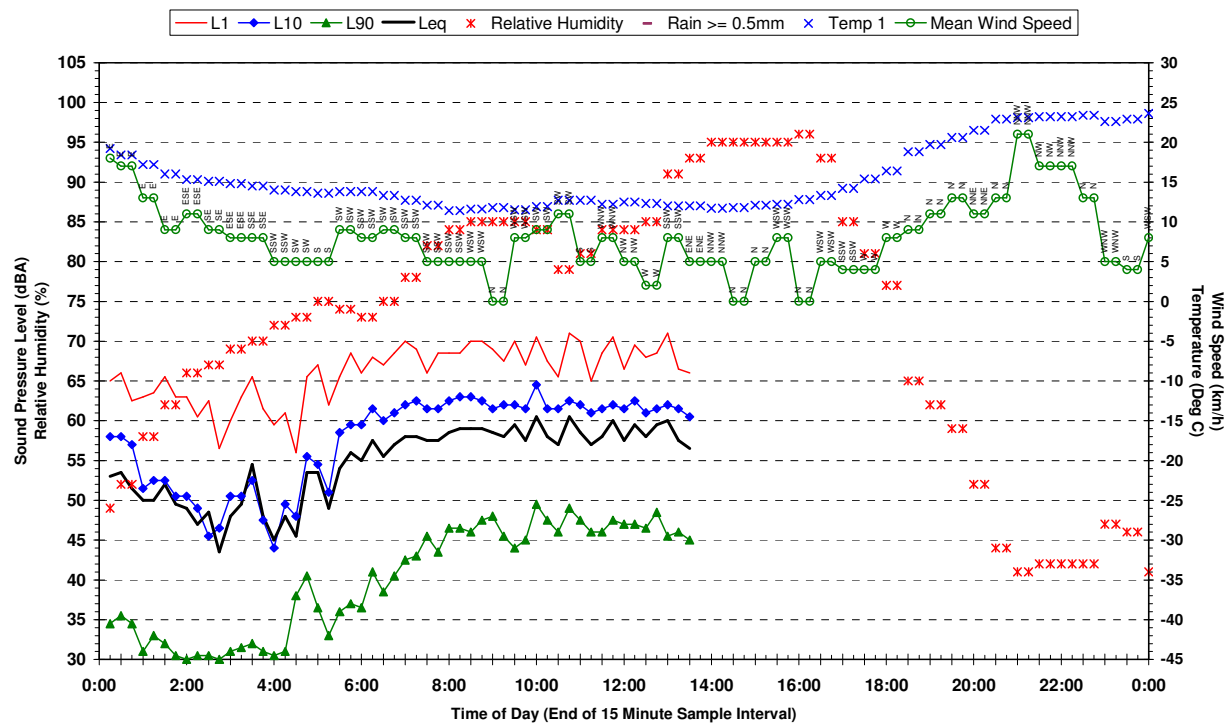
Statistical Ambient Noise Levels BG1 - 615 Bringelly Rd Rossmore - Saturday 29 April 2006
