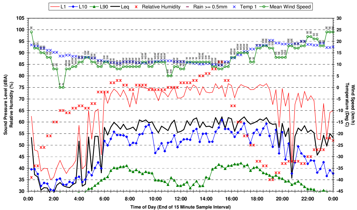
Statistical Ambient Noise Levels BG2 - 198 McCann Rd Rossmore - Monday 24 April 2006
