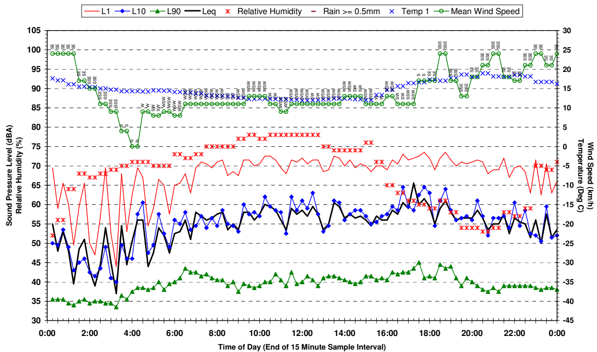
Statistical Ambient Noise Levels 18 Newtown Rd Glenfield - Tuesday 25 April 2006
