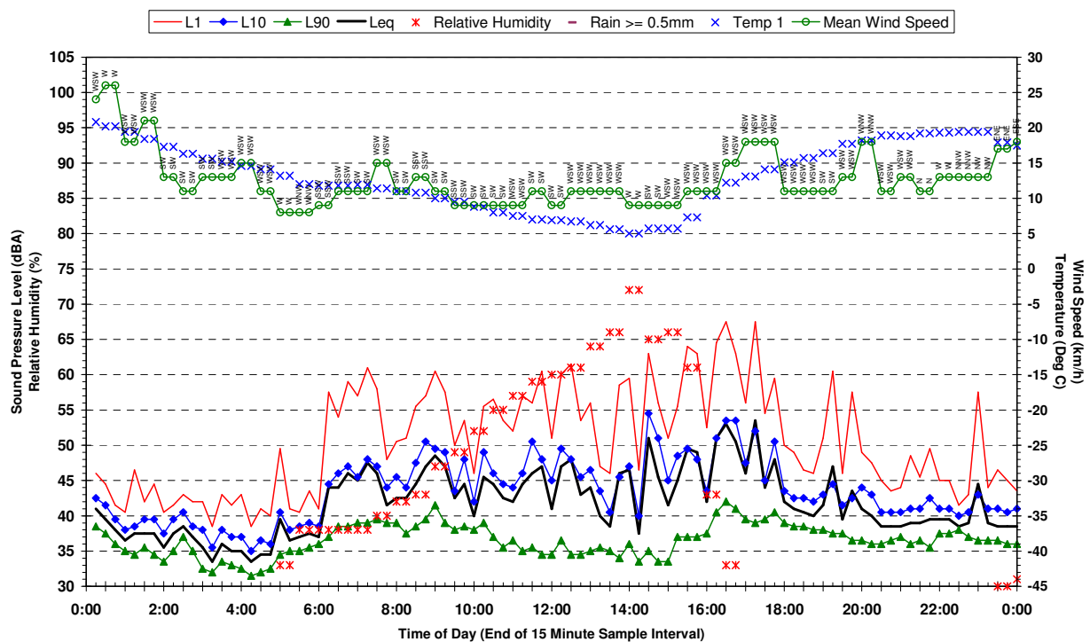
Statistical Ambient Noise Levels 25 Cassidy St Denham Court - Saturday 22 April 2006
