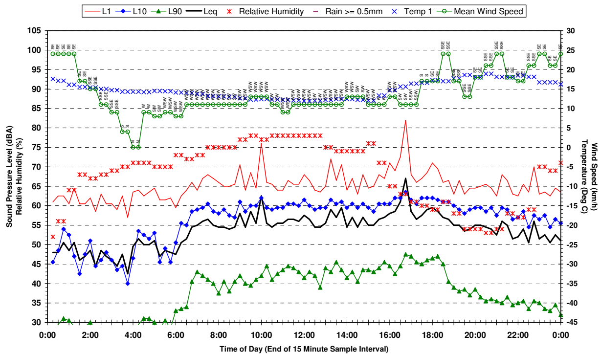
Statistical Ambient Noise Levels BG1 - 615 Bringelly Rd Rossmore - Tuesday 25 April 2006
