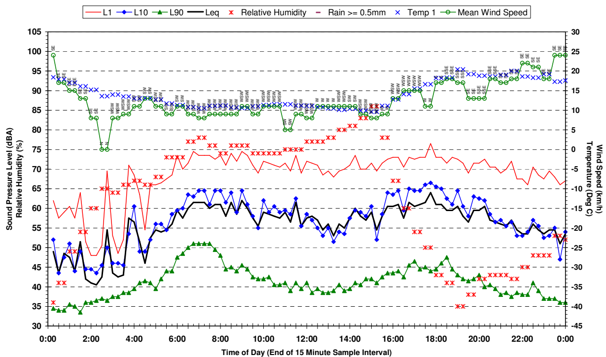
Statistical Ambient Noise Levels 18 Newtown Rd Glenfield - Monday 24 April 2006
