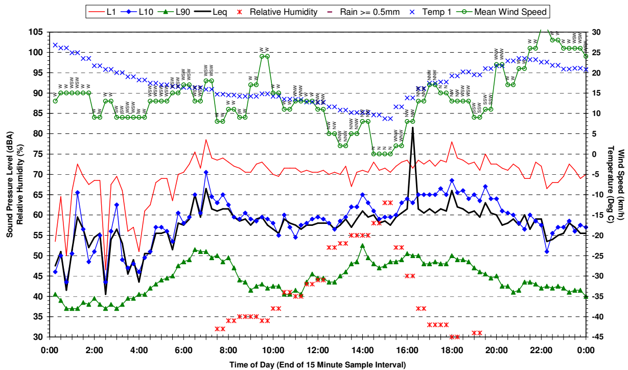
Statistical Ambient Noise Levels 18 Newtown Rd Glenfield - Friday 21 April 2006
