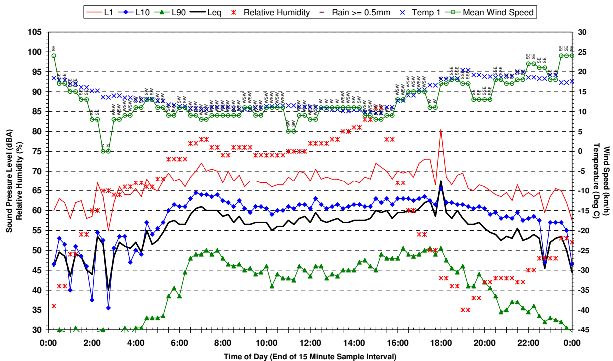
Statistical Ambient Noise Levels BG1 - 615 Bringelly Rd Rossmore - Monday 24 April 2006
