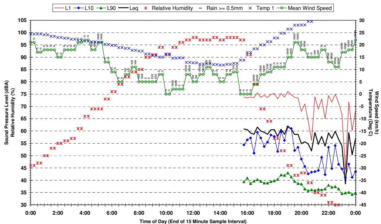
Statistical Ambient Noise Levels BG2 - 198 McCann Rd Rossmore - Wednesday 19 April 2006
