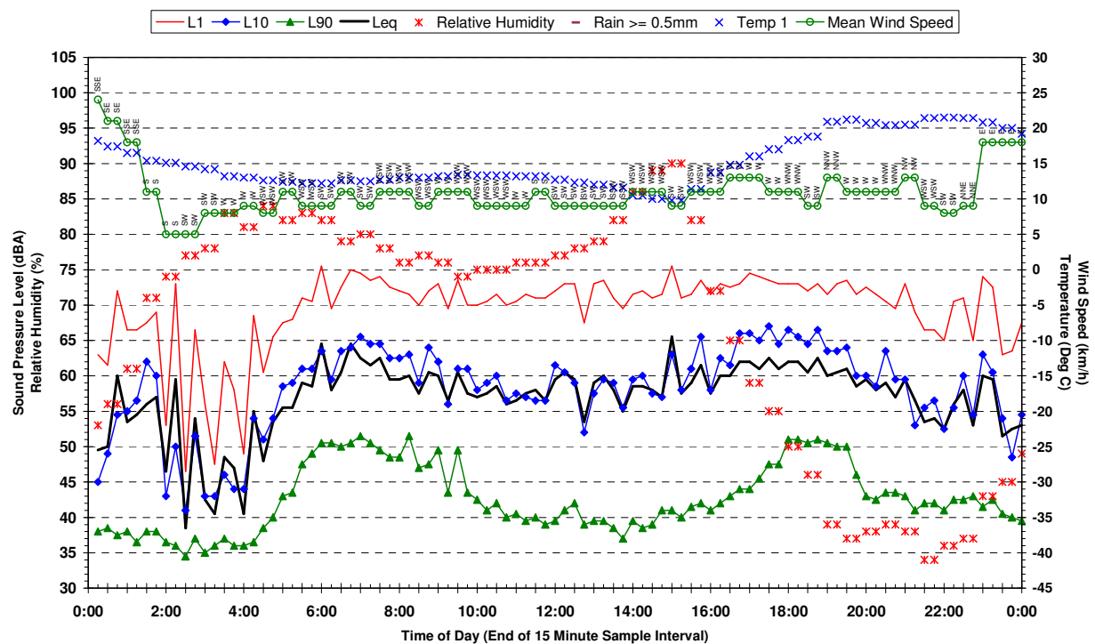
Statistical Ambient Noise Levels 18 Newtown Rd Glenfield - Friday 28 April 2006
