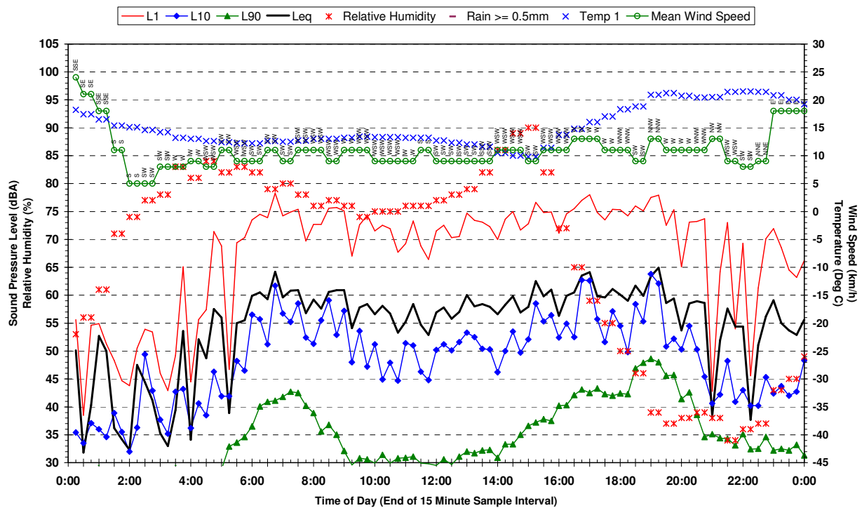
Statistical Ambient Noise Levels BG2 - 198 McCann Rd Rossmore - Friday 28 April 2006
